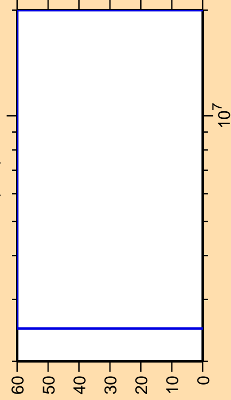
\Delta\sigma/\sigma vs. E for ^{145}\text{Tb}(n,d)
