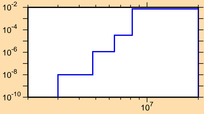
\sigma vs. E for ^{145}\text{Tb}(n,d)
