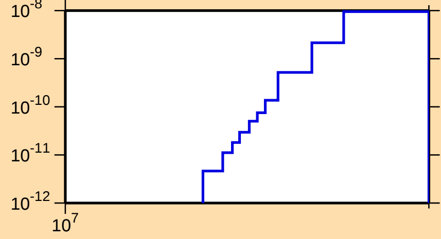
\sigma vs. E for ^{146}\text{Tb}(\text{mt117})
