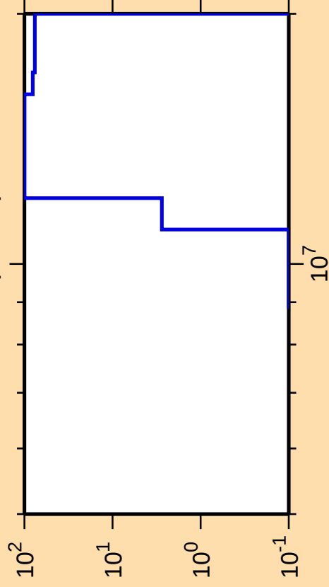
\Delta\sigma/\sigma vs. E for ^{146}\text{Tb}(\text{mt } 45)
