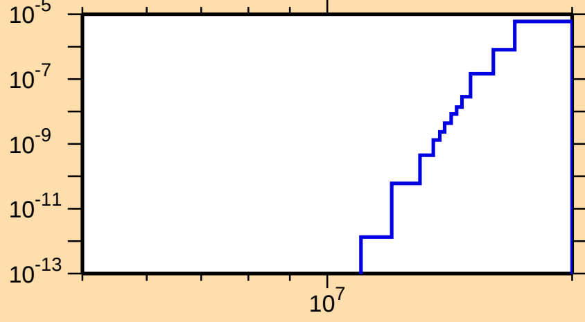
\sigma vs. E for ^{146}\text{Tb}(\text{mt } 45)
