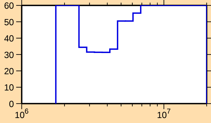
\Delta\sigma/\sigma vs. E for ^{146}\text{Tb}(n,n\text{cont.})
