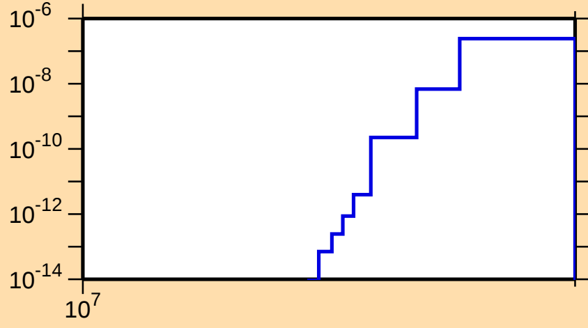
\sigma vs. E for ^{146}\text{Tb}(n,2n\alpha)
