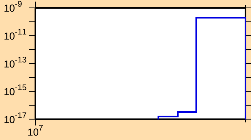
\sigma vs. E for ^{146}\text{Tb}(n,\text{nt})
