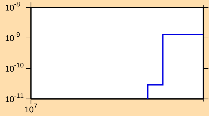
\sigma vs. E for ^{146}\text{Tb}(\text{mt } 34)
