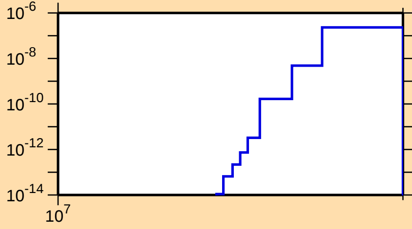
\sigma vs. E for ^{146}\text{Tb}(n,\text{pt})
