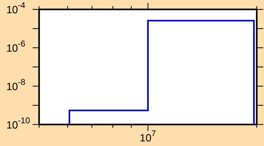
\sigma vs. E for ^{146}\text{Tb}(n,\text{He3})
