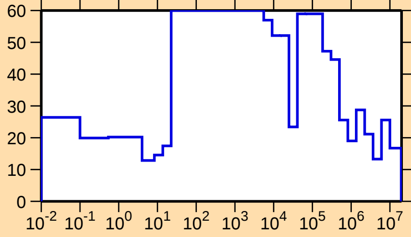
\Delta\sigma/\sigma vs. E for ^{146}\text{Tb}(n,\text{tot.})
