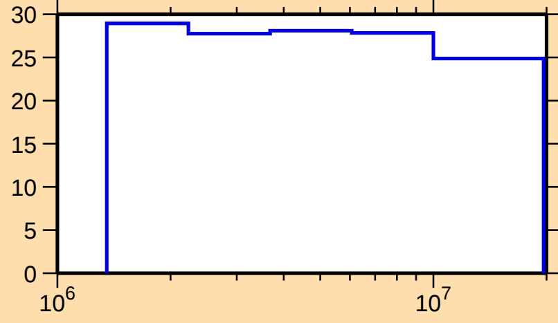
\Delta\sigma/\sigma vs. E for ^{146}\text{Tb}(n,\text{nonel.})
