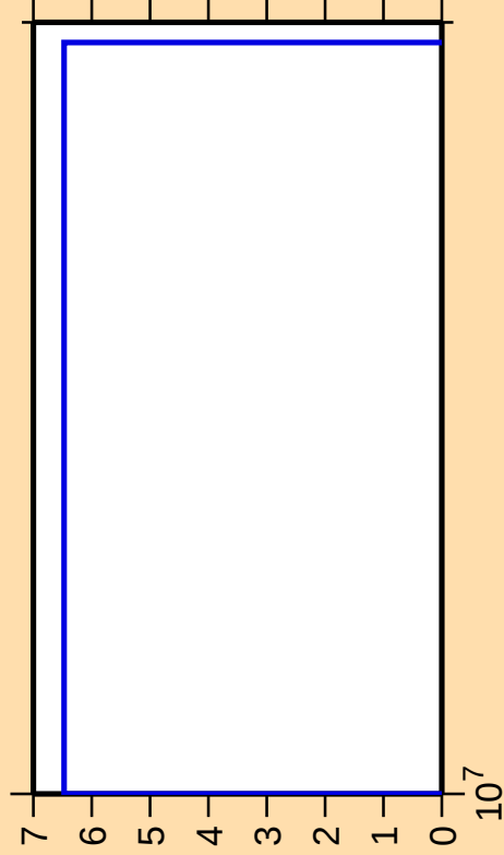
\Delta\sigma/\sigma vs. E for ^{146}\text{Tb}(n,\text{nt})
