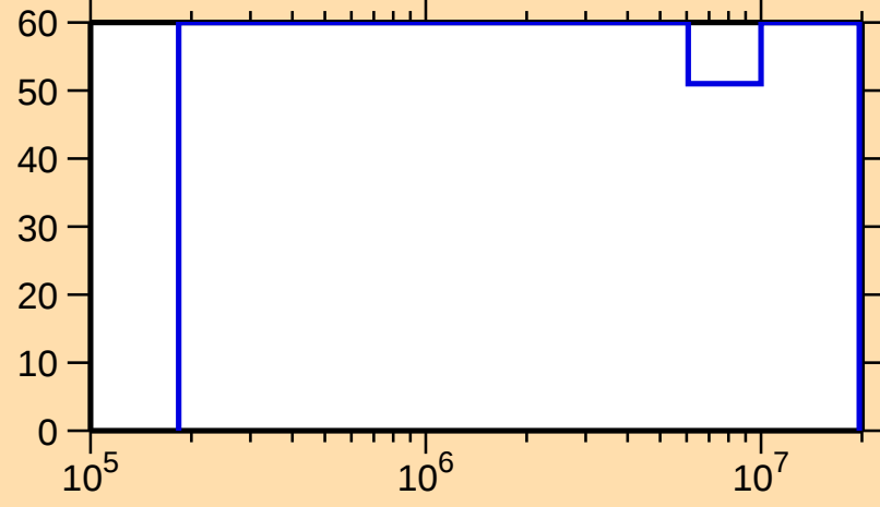
\Delta\sigma/\sigma vs. E for ^{146}\text{Tb}(n,n_1)
