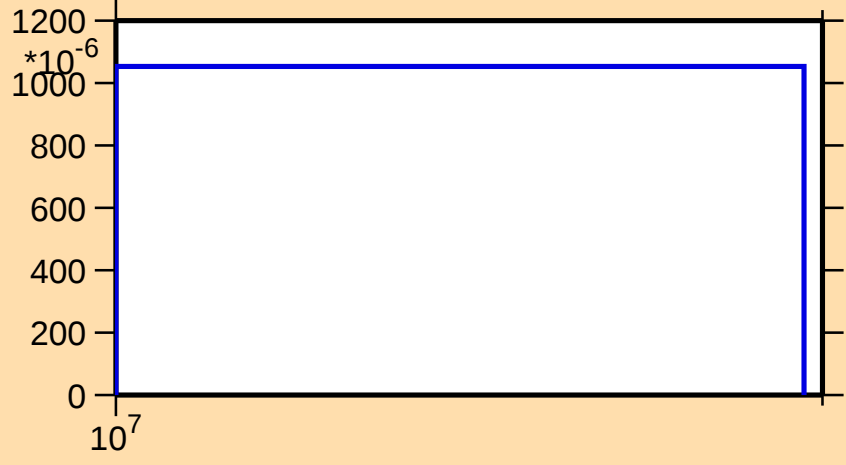
\sigma vs. E for ^{146}\text{Tb}(n,2np)
