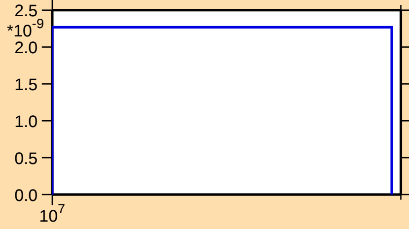
\sigma vs. E for ^{146}\text{Tb}(n,\text{pt})
