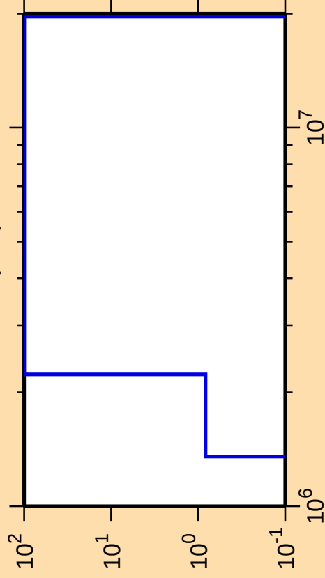
\Delta\sigma/\sigma vs. E for ^{146}\text{Tb}(n,d)
