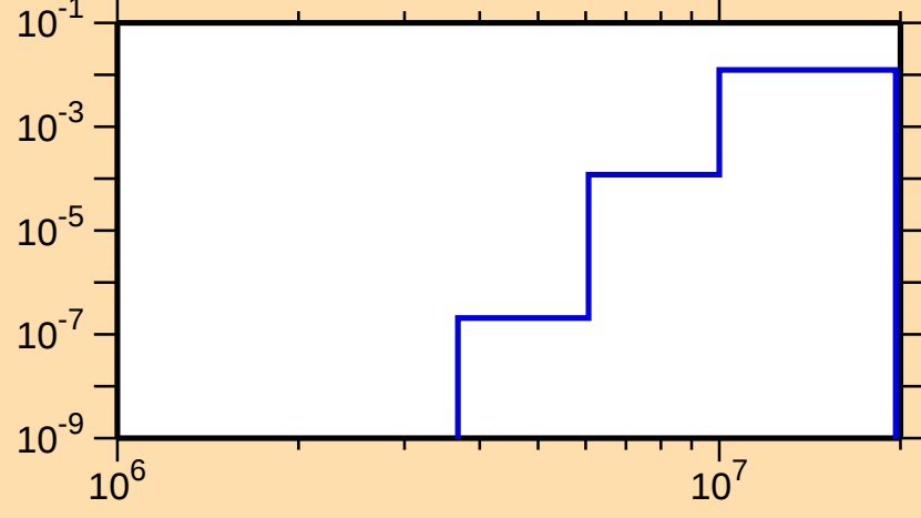
\sigma vs. E for ^{146}\text{Tb}(n,d)
