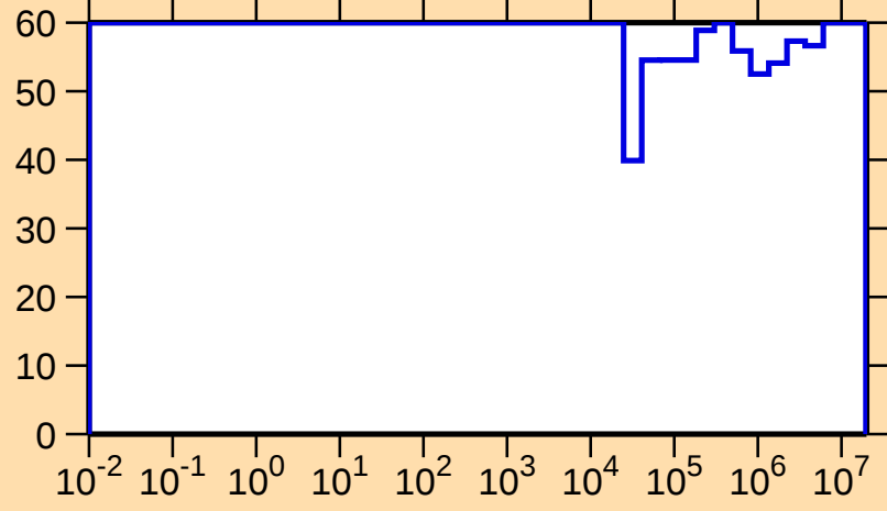
\Delta\sigma/\sigma vs. E for ^{146}\text{Tb}(n,p)
