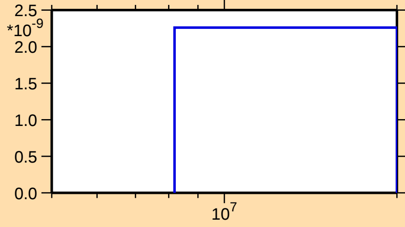
\sigma vs. E for ^{146}\text{Tb}(n,2n\alpha)
