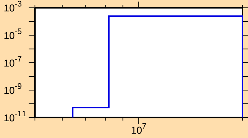
\sigma vs. E for ^{146}\text{Tb}(n,t)
