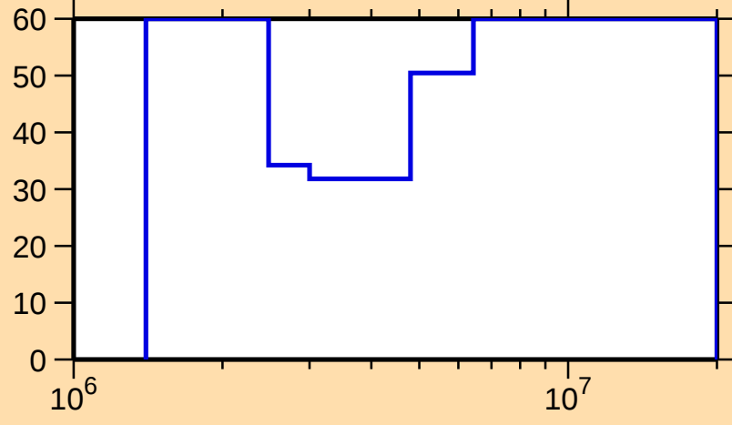
\Delta\sigma/\sigma vs. E for ^{146}\text{Tb}(n,ncont.)
