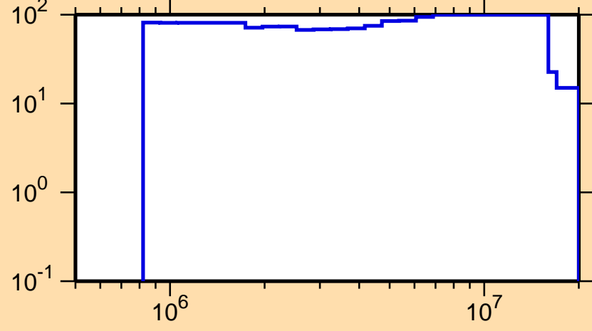
\Delta\sigma/\sigma vs. E for ^{146}\text{Tb}(n,n_1)
