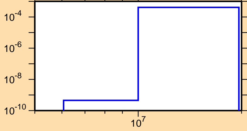
\sigma vs. E for ^{146}\text{Tb}(n,t)
