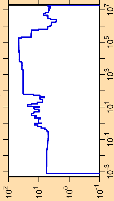
\Delta\sigma/\sigma vs. E for ^{147}\text{Tb}(n,\text{tot.})
