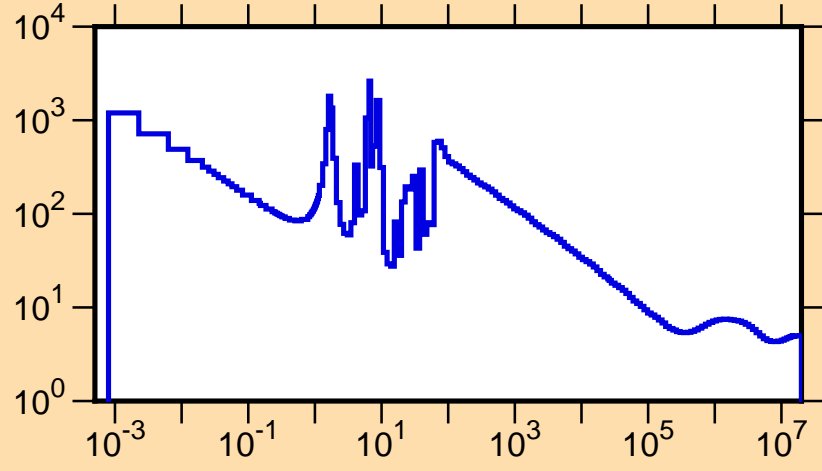
\sigma vs. E for ^{147}\text{Tb}(n,\text{tot.})
