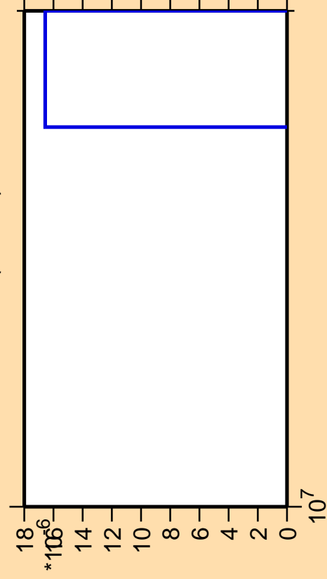
\Delta\sigma/\sigma vs. E for ^{148}\text{Tb} (mt 11)
