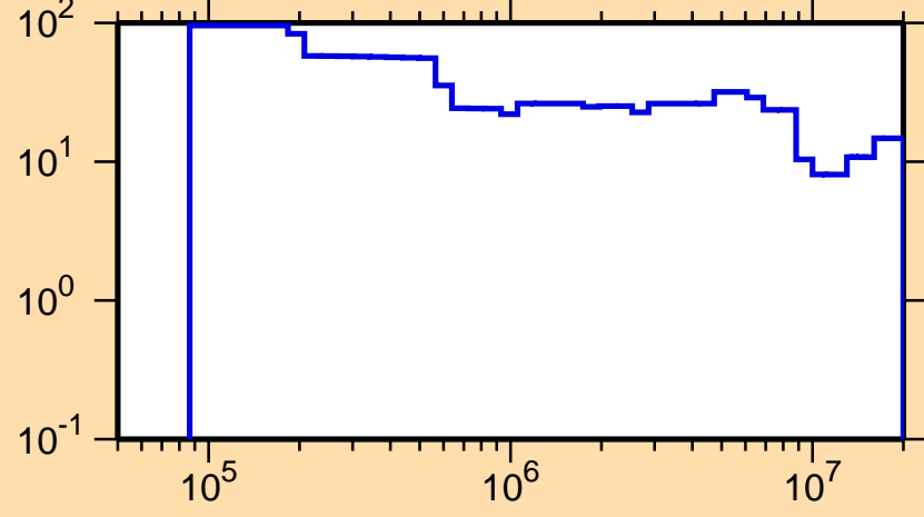
\Delta\sigma/\sigma vs. E for ^{148}\text{Tb}(n,\text{tot.})
