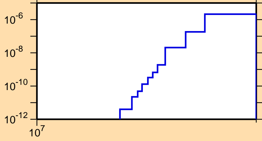
\sigma vs. E for ^{148}\text{Tb}(n,2n\alpha)
