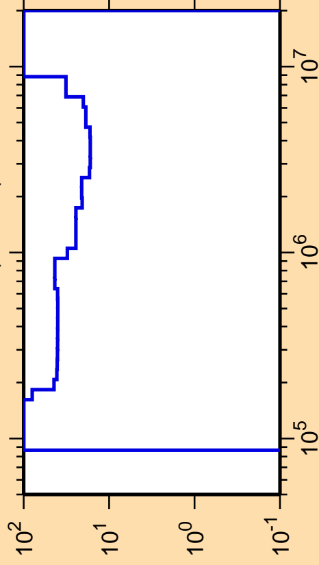
\Delta\sigma/\sigma vs. E for ^{148}\text{Tb}(n,\text{inel.})
