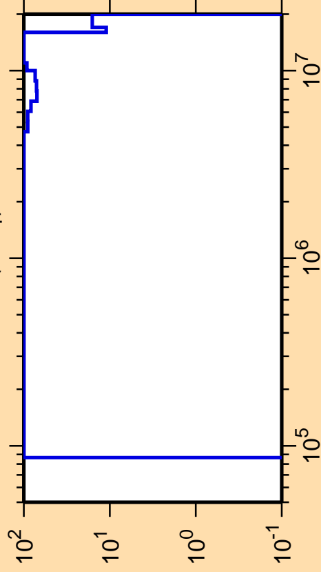
\Delta\sigma/\sigma vs. E for ^{148}\text{Tb}(n,n_1)
