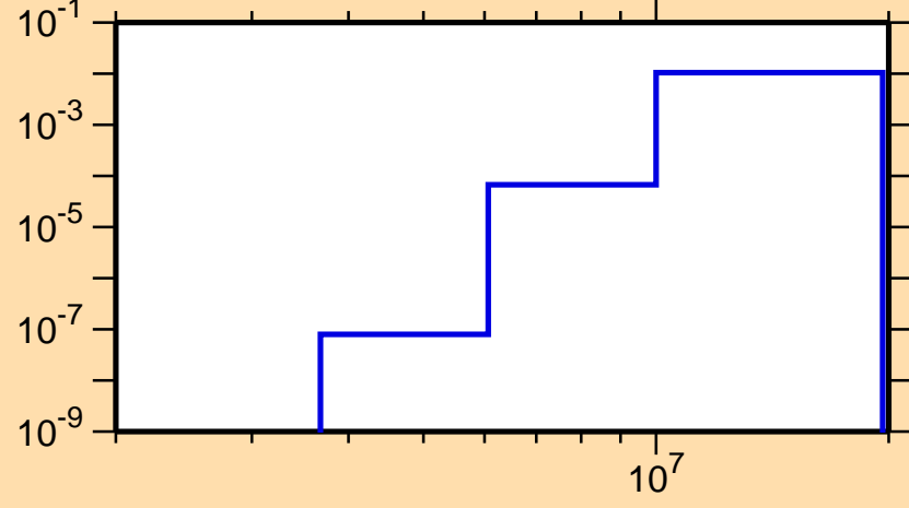
\sigma vs. E for ^{148}\text{Tb}(n,d)
