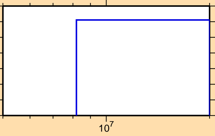
\sigma vs. E for ^{148}\text{Tb}(\text{mt117})
