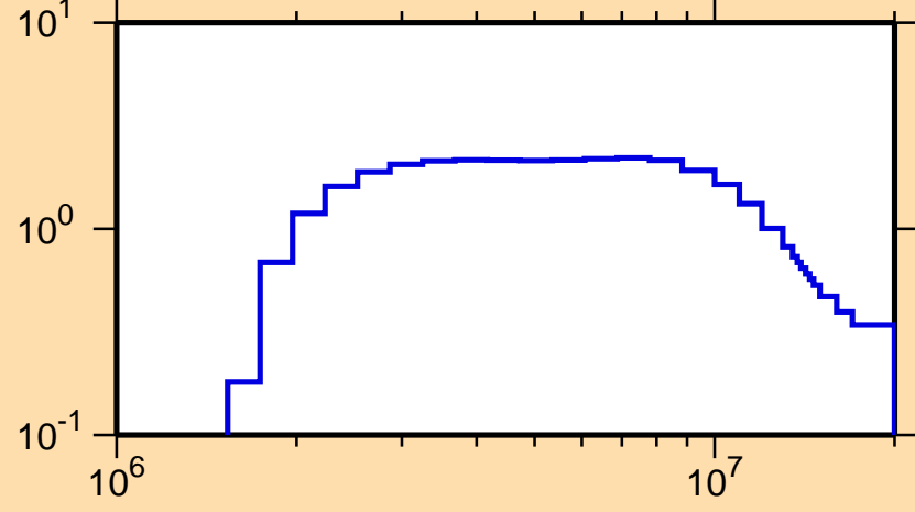
\sigma vs. E for ^{148}\text{Tb}(n,n\text{cont.})
