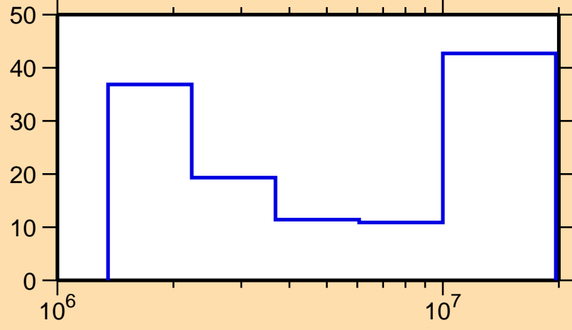
\Delta\sigma/\sigma vs. E for ^{148}\text{Tb}(n,ncont.)
