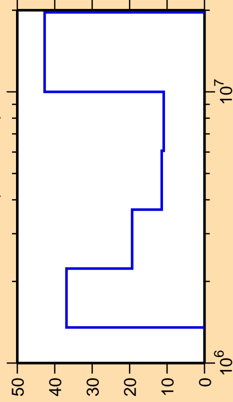
\Delta\sigma/\sigma vs. E for ^{148}\text{Tb}(n,\text{ncont.})
