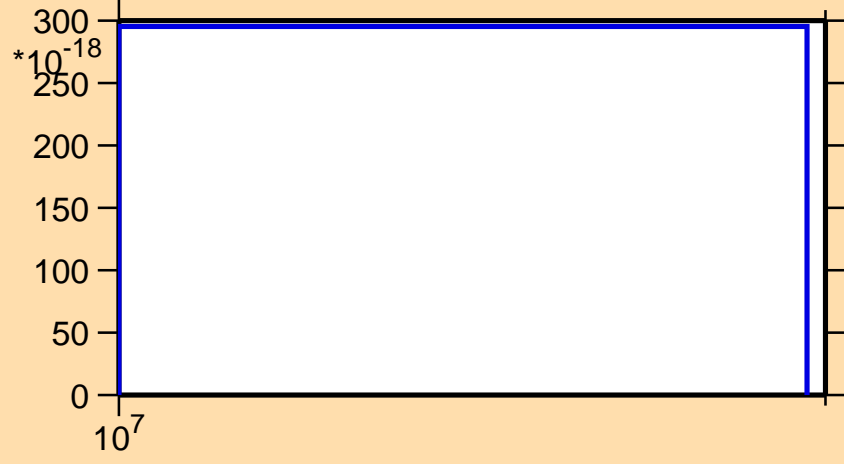
\sigma vs. E for ^{149}\text{Tb} (mt 11)
