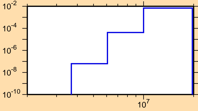
\sigma vs. E for ^{149}\text{Tb}(n,d)
