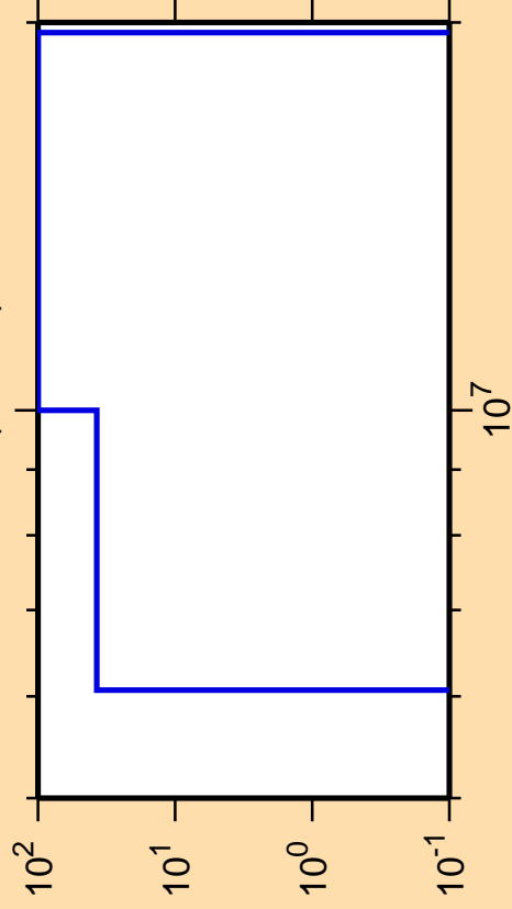
\Delta\sigma/\sigma vs. E for ^{149}\text{Tb}(\text{mt } 45)
