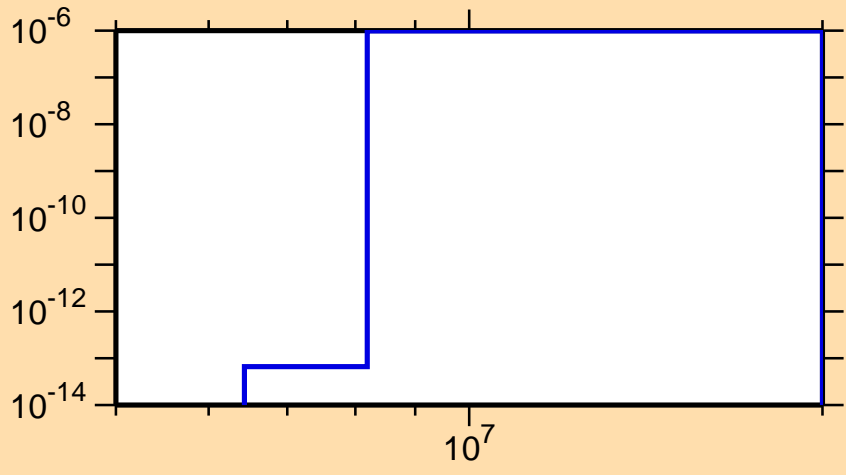
\sigma vs. E for ^{149}\text{Tb}(\text{mt } 45)
