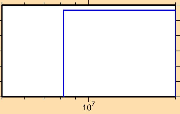
\sigma vs. E for ^{149}\text{Tb}(n,\text{nd})
