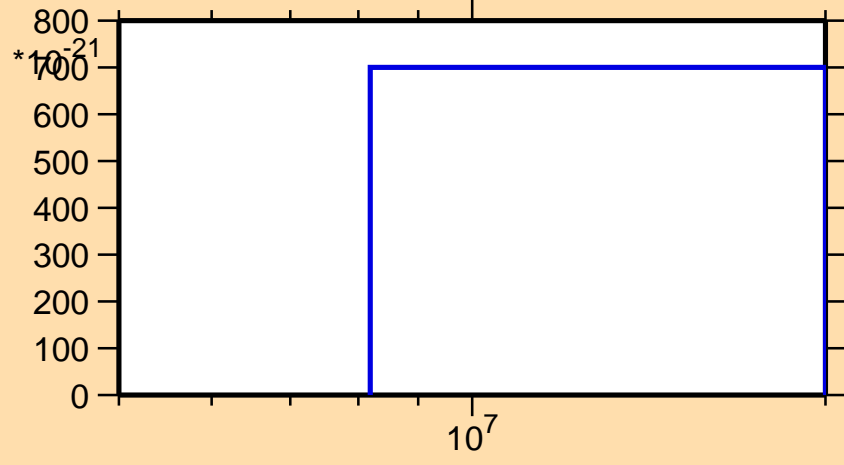
\sigma vs. E for ^{149}\text{Tb}(\text{mt } 42)
