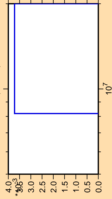
\Delta\sigma/\sigma vs. E for ^{149}\text{Tb} (mt 11)
