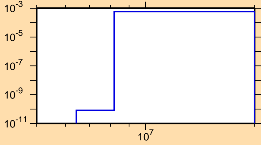
\sigma vs. E for ^{149}\text{Tb}(n,t)
