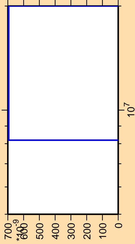
\Delta\sigma/\sigma vs. E for ^{149}\text{Tb}(\text{mt } 42)
