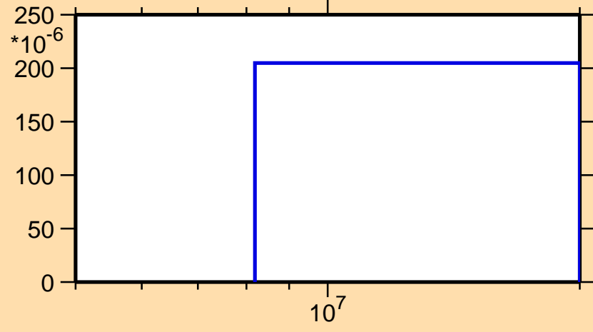
\sigma vs. E for ^{149}\text{Tb}(n,2np)
