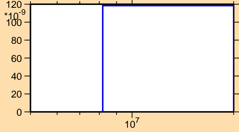
\sigma vs. E for ^{149}\text{Tb}(n,2n\alpha)
