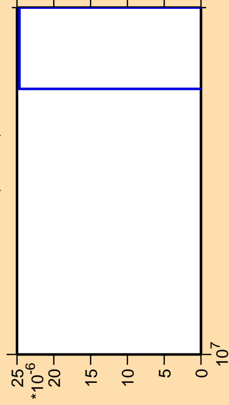
\Delta\sigma/\sigma vs. E for ^{149}\text{Tb} (mt 42)
