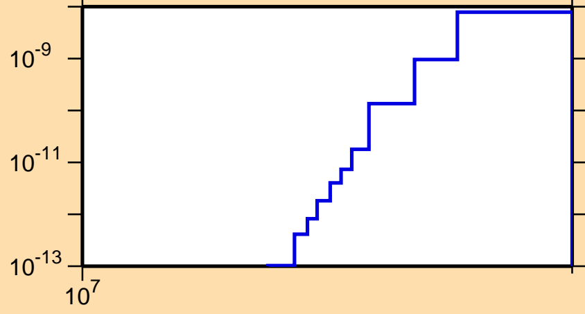
\sigma vs. E for ^{149}\text{Tb}(n,\text{pd})
