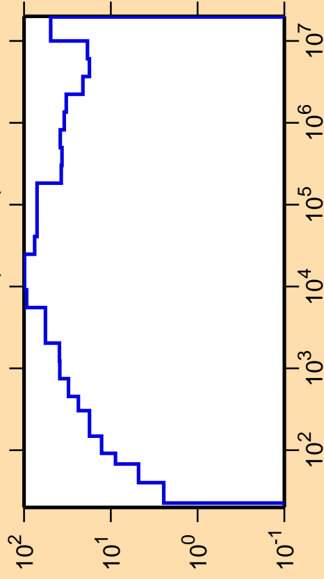
\Delta\sigma/\sigma vs. E for ^{149}\text{Tb}(n,\text{inel.})
