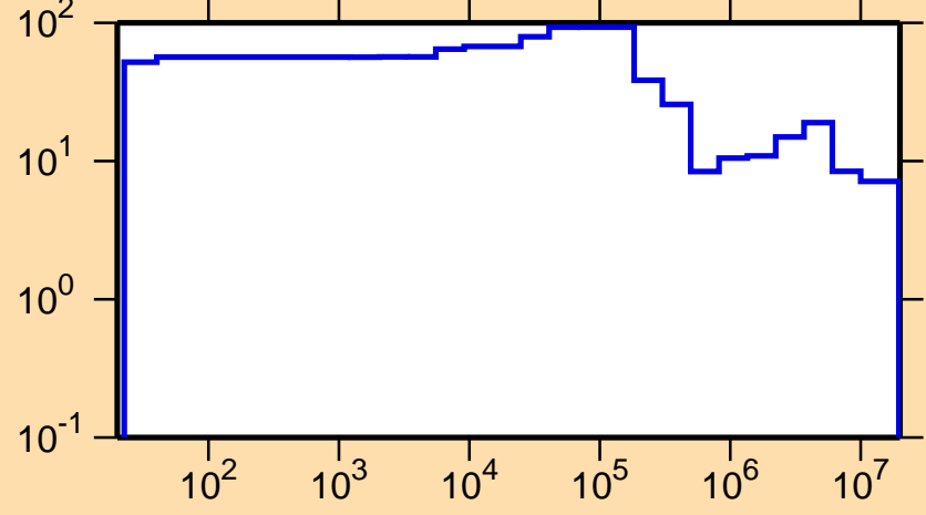
\Delta\sigma/\sigma vs. E for ^{149}\text{Tb}(n,\text{el.})
