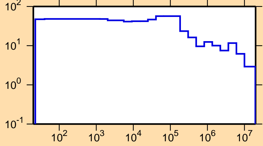
\Delta\sigma/\sigma vs. E for ^{149}\text{Tb}(n,\text{tot.})
