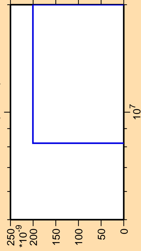
\Delta\sigma/\sigma vs. E for ^{149}\text{Tb}(\text{mt } 42)
