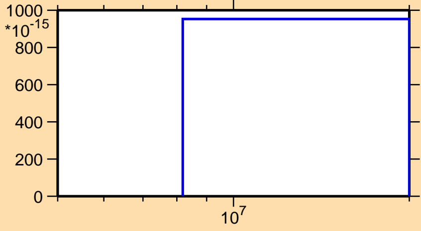
\sigma vs. E for ^{149}\text{Tb}(\text{mt } 34)
