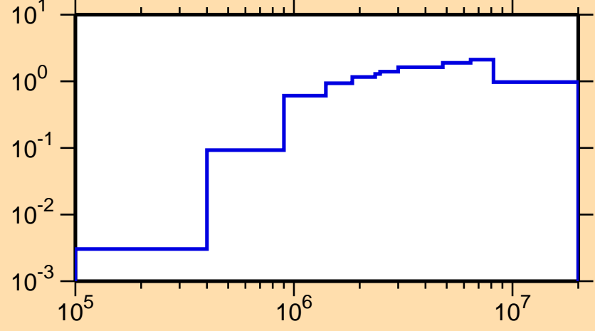
\sigma vs. E for ^{149}\text{Tb}(n,\text{inel.})
