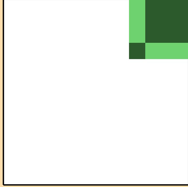
\sigma vs. E for ^{150}\text{Tb}(n,3n)
