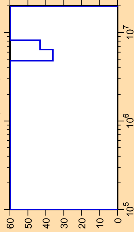
\Delta\sigma/\sigma vs. E for ^{150}\text{Tb}(n,\text{inel.})
