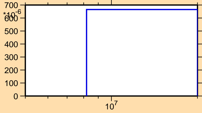
\sigma vs. E for ^{150}\text{Tb}(n,2np)
