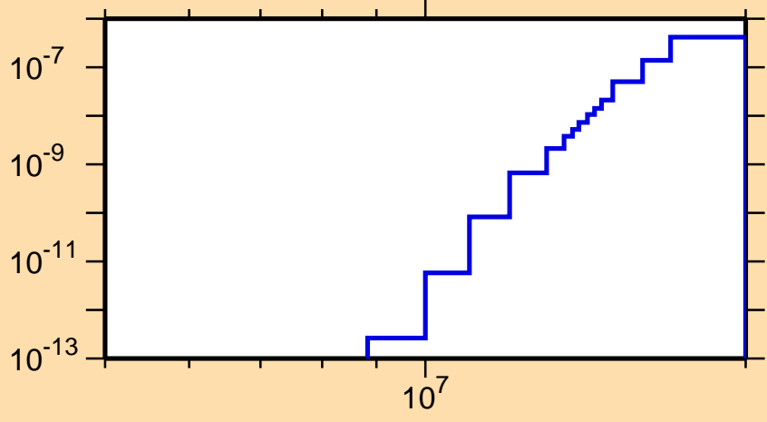
\sigma vs. E for ^{150}\text{Tb} (mt 45)
