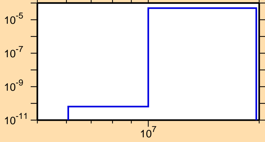
\sigma vs. E for ^{150}\text{Tb}(n,2n\alpha)
