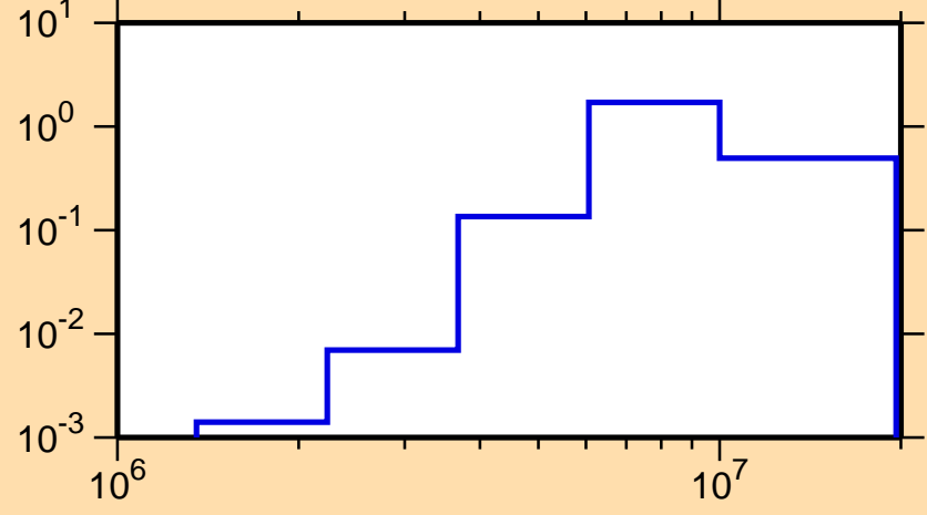
\sigma vs. E for ^{150}\text{Tb}(n,n\text{cont.})
