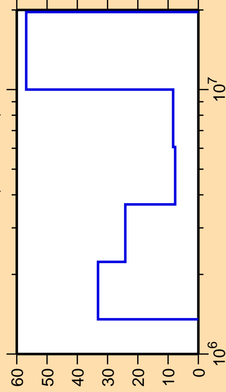
\Delta\sigma/\sigma vs. E for ^{150}\text{Tb}(n,n\text{cont.})
