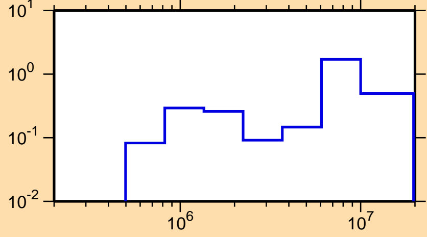
\sigma vs. E for ^{150}\text{Tb}(n,\text{inel.})
