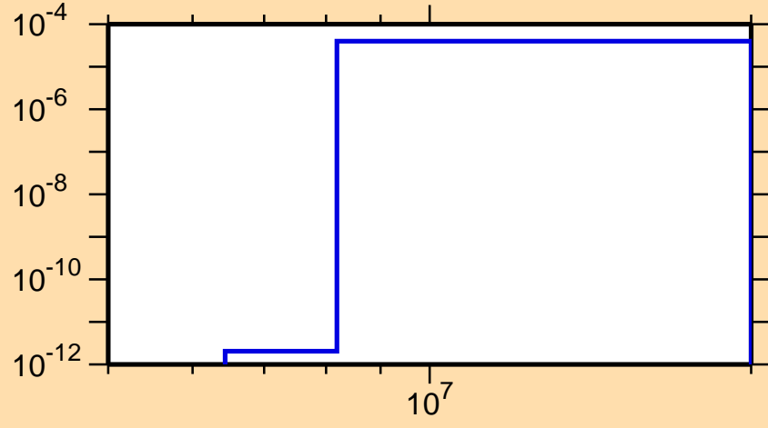
\sigma vs. E for ^{150}\text{Tb}(n,2n\alpha)
