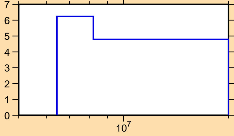
\Delta\sigma/\sigma vs. E for ^{150}\text{Tb}(n,\text{el.})
