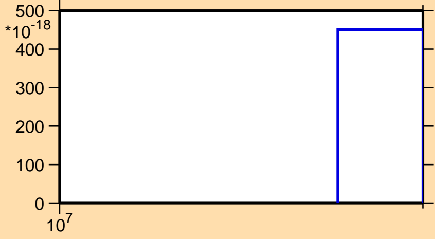
\sigma vs. E for ^{151}\text{Tb} (mt 42)
