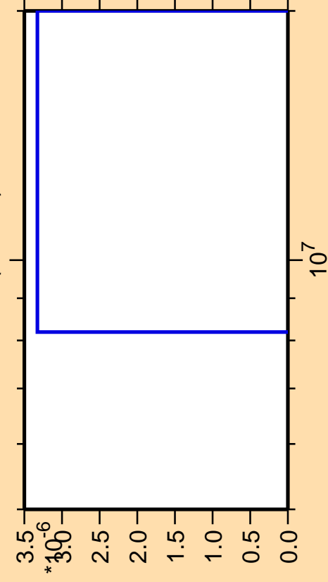
\Delta\sigma/\sigma vs. E for ^{151}\text{Tb} (mt 42)
