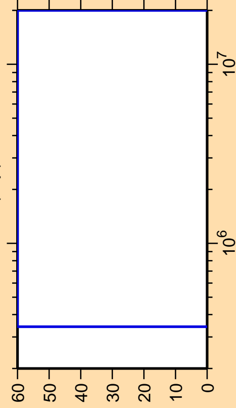
\Delta\sigma/\sigma vs. E for ^{152}\text{Tb}(n,p)
