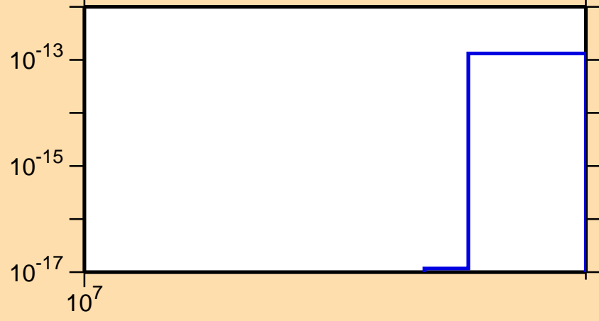
\sigma vs. E for ^{152}\text{Tb} (mt 11)
