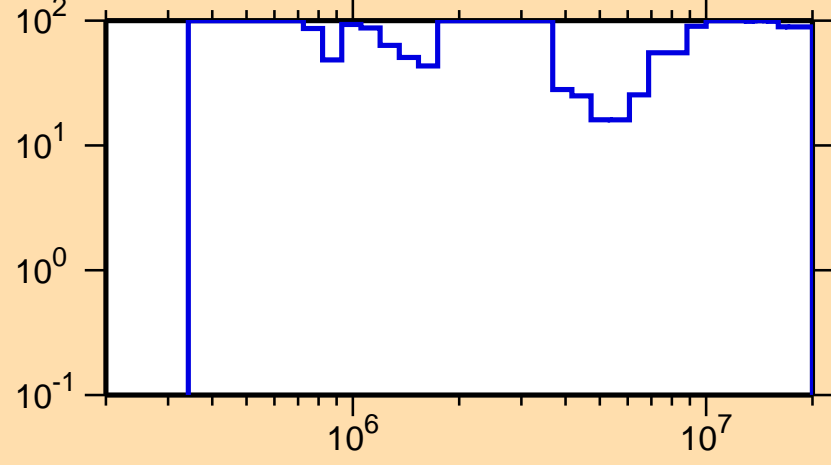
\Delta\sigma/\sigma vs. E for ^{152}\text{Tb}(n,ncont.)
