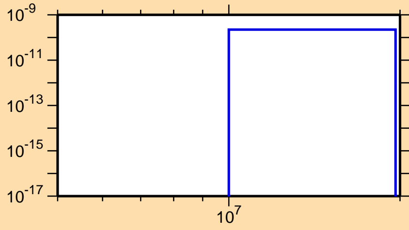
\sigma vs. E for ^{152}\text{Tb}(\text{mt117})
