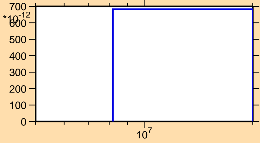
\sigma vs. E for ^{152}\text{Tb}(\text{mt } 45)
