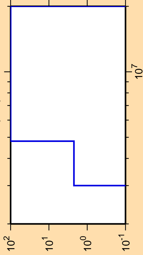
\Delta\sigma/\sigma vs. E for ^{152}\text{Tb}(n,d)
