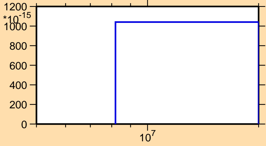
\sigma vs. E for ^{152}\text{Tb}(\text{mt } 34)
