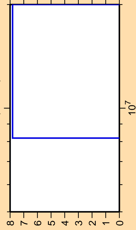
\Delta\sigma/\sigma vs. E for ^{152}\text{Tb}(\text{mt } 34)
