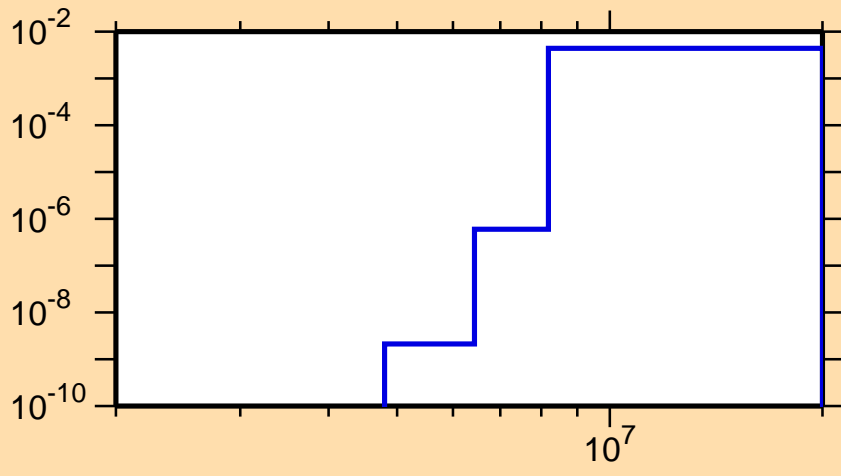
\sigma vs. E for ^{152}\text{Tb}(n,d)
