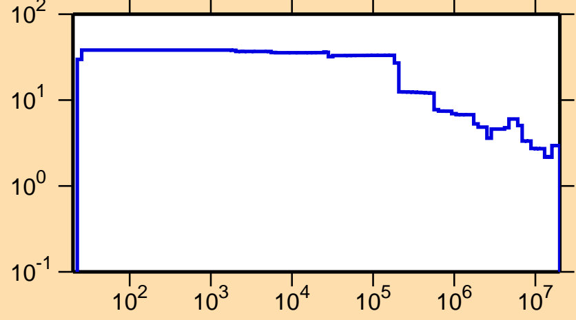
\Delta\sigma/\sigma vs. E for ^{152}\text{Tb}(n,\text{tot.})
