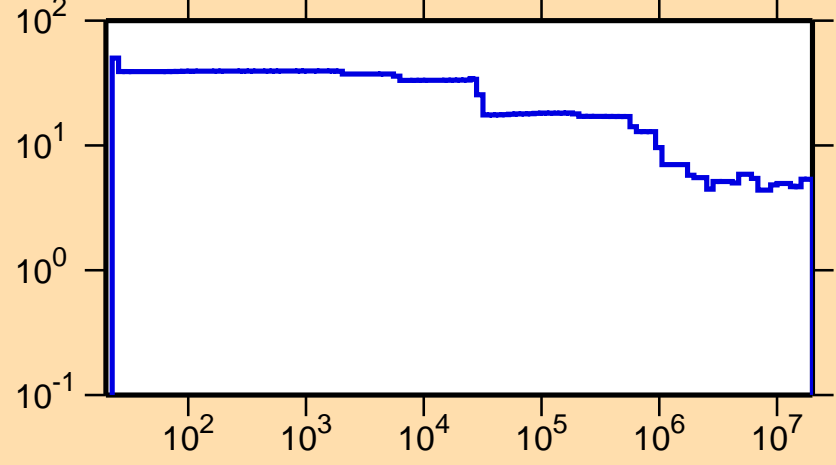
\Delta\sigma/\sigma vs. E for ^{152}\text{Tb}(n,\text{nonel.})
