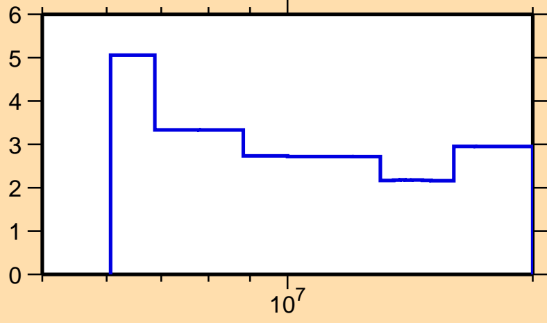
\Delta\sigma/\sigma vs. E for ^{152}\text{Tb}(n,tot.)
