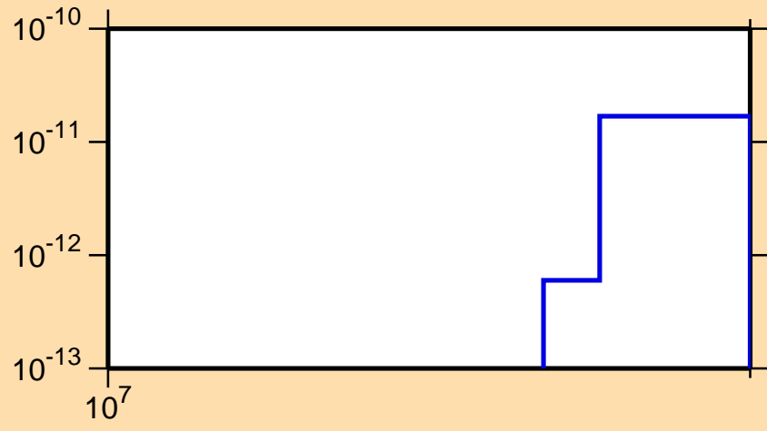
\sigma vs. E for ^{152}\text{Tb}(n,\text{pd})
