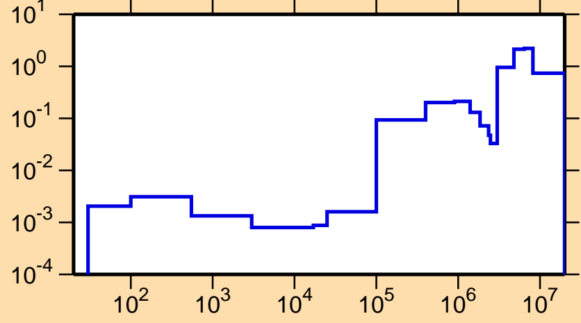
\sigma vs. E for ^{152}\text{Tb}(n,\text{inel.})
