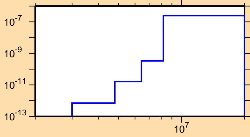
\sigma vs. E for ^{152}\text{Tb}(n,p\alpha)
