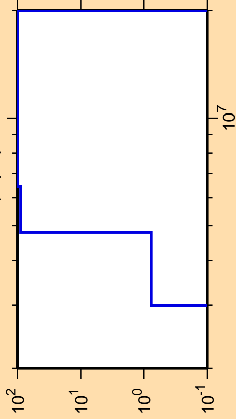
\Delta\sigma/\sigma vs. E for ^{152}\text{Tb}(n,p\alpha)
