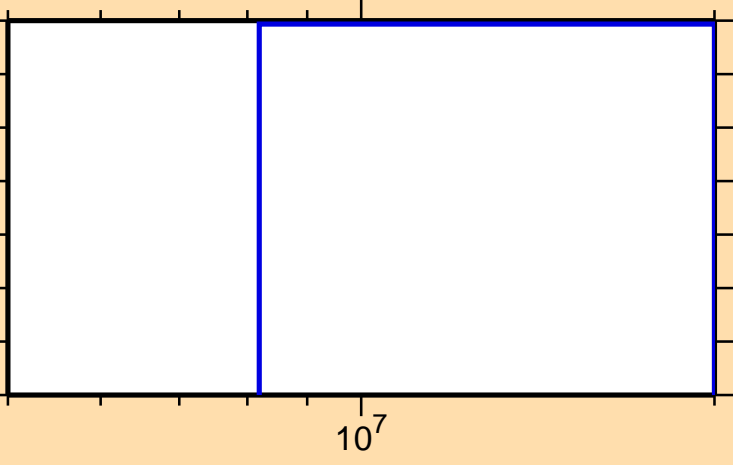
\sigma vs. E for ^{152}\text{Tb}(n,3n)
