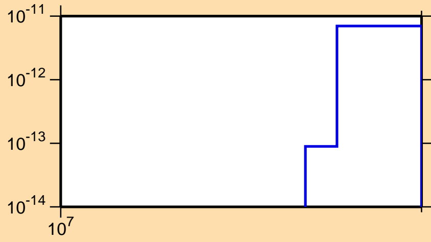
\sigma vs. E for ^{153}\text{Tb}(n,3n\alpha)
