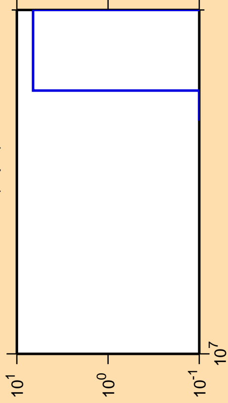
\Delta\sigma/\sigma vs. E for ^{153}\text{Tb}(n,\text{pd})
