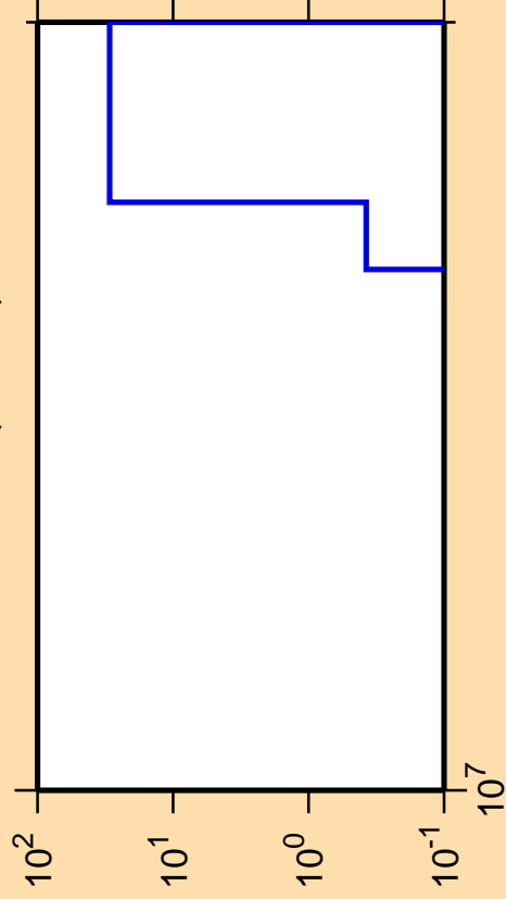
\Delta\sigma/\sigma vs. E for ^{153}\text{Tb}(n,3n\alpha)
