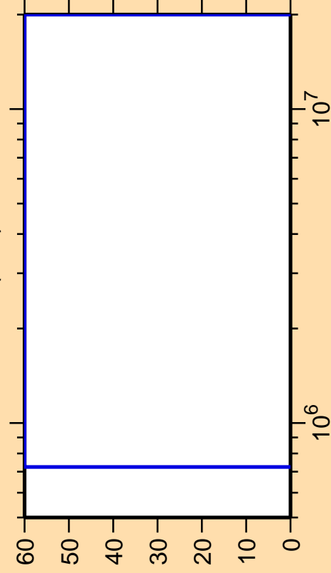
\Delta\sigma/\sigma vs. E for ^{153}\text{Tb}(n,\alpha)
