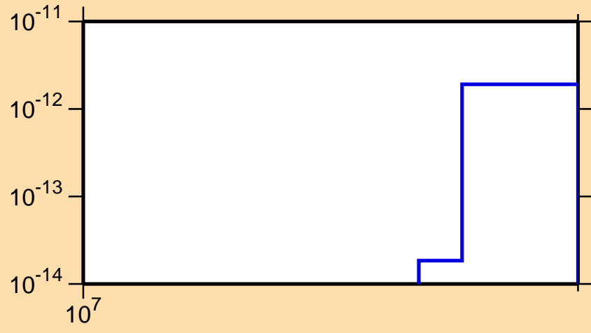
\sigma vs. E for ^{153}\text{Tb}(n,\text{pd})
