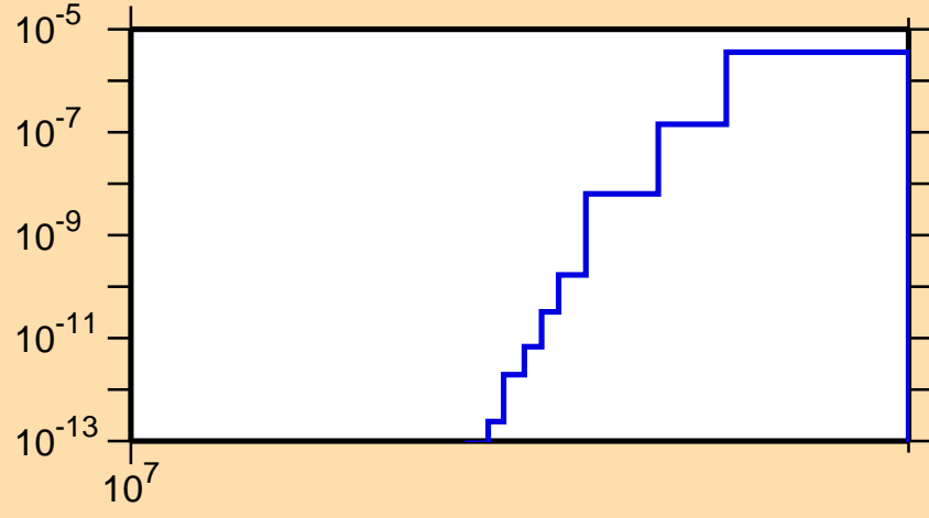
\sigma vs. E for ^{153}\text{Tb}(n,nt)
