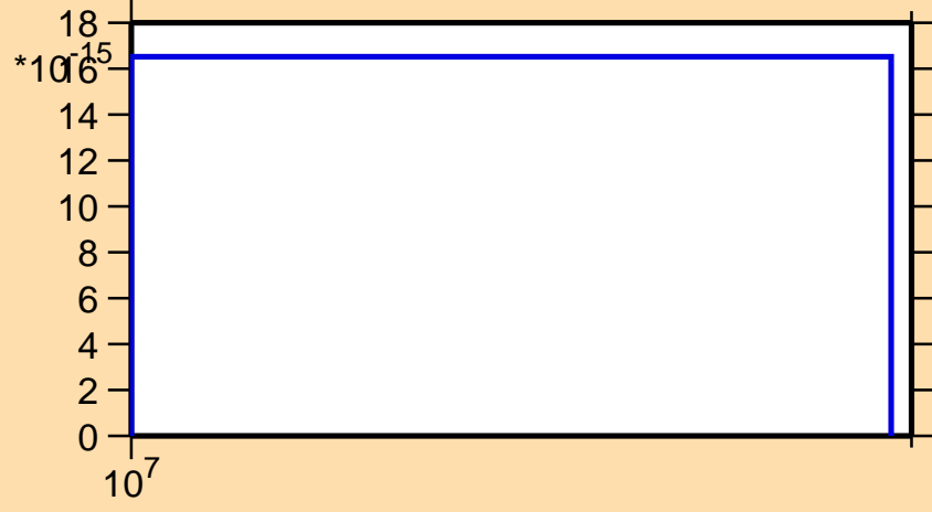
\sigma vs. E for ^{153}\text{Tb}(n,\text{pd})
