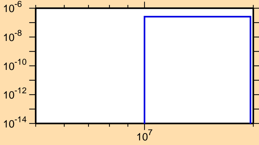
\sigma vs. E for ^{153}\text{Tb}(n,2n\alpha)
