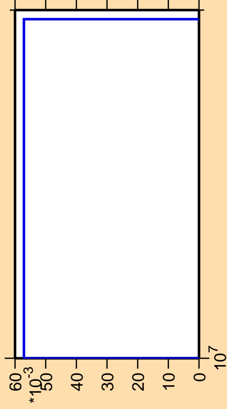
\Delta\sigma/\sigma vs. E for ^{153}\text{Tb}(n,\text{pd})
