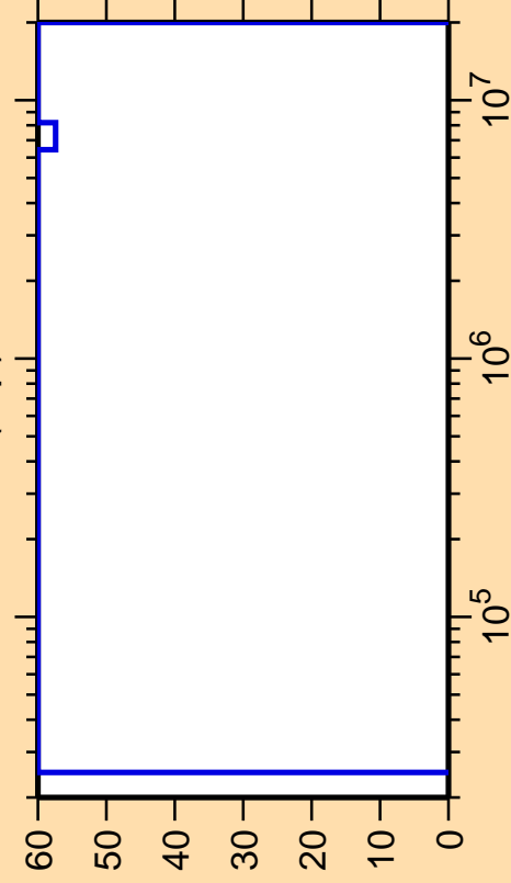
\Delta\sigma/\sigma vs. E for ^{153}\text{Tb}(n,p)
