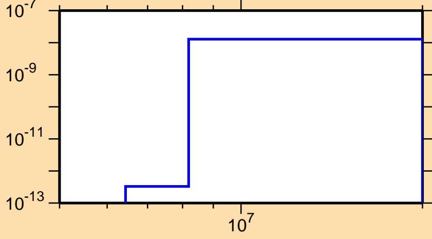
\sigma vs. E for ^{153}\text{Tb}(n,p\alpha)
