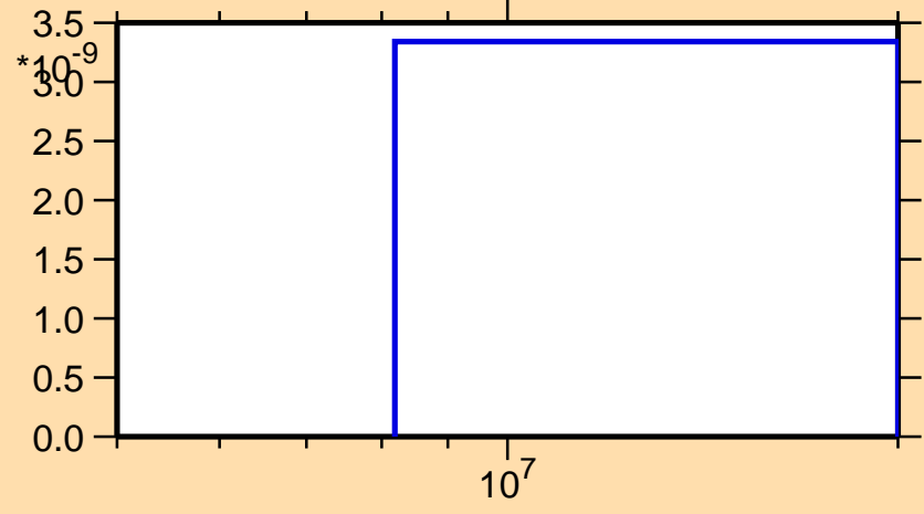
\sigma vs. E for ^{153}\text{Tb}(n,\text{He3})
