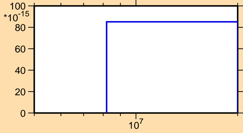
\sigma vs. E for ^{153}\text{Tb}(n,3n\alpha)
