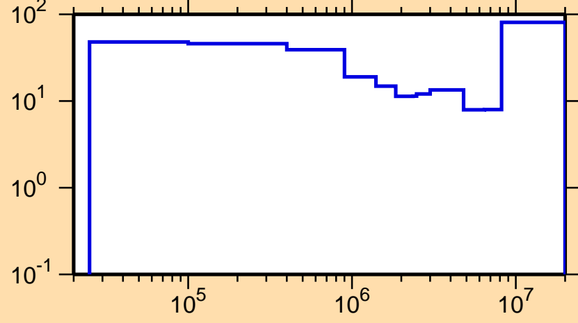
\Delta\sigma/\sigma vs. E for ^{153}\text{Tb}(n,\text{inel.})
