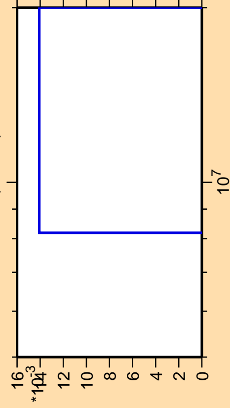
\Delta\sigma/\sigma vs. E for ^{153}\text{Tb} (mt 34)
