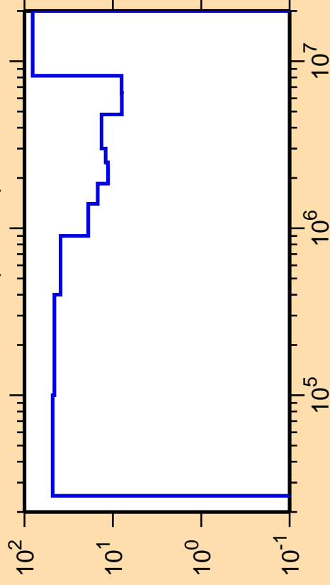
\Delta\sigma/\sigma vs. E for ^{153}\text{Tb}(n,\text{inel.})
