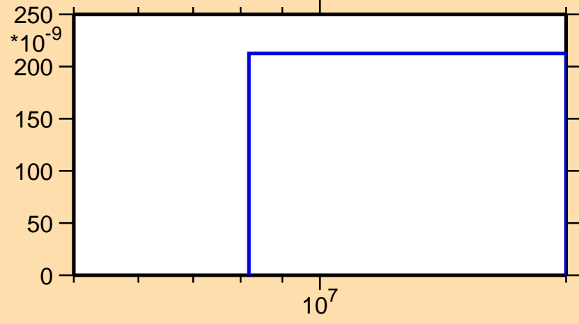
\sigma vs. E for ^{153}\text{Tb}(n,2n\alpha)
