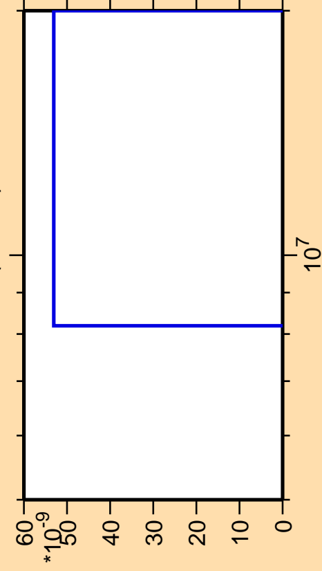
\Delta\sigma/\sigma vs. E for ^{153}\text{Tb} (mt 42)
