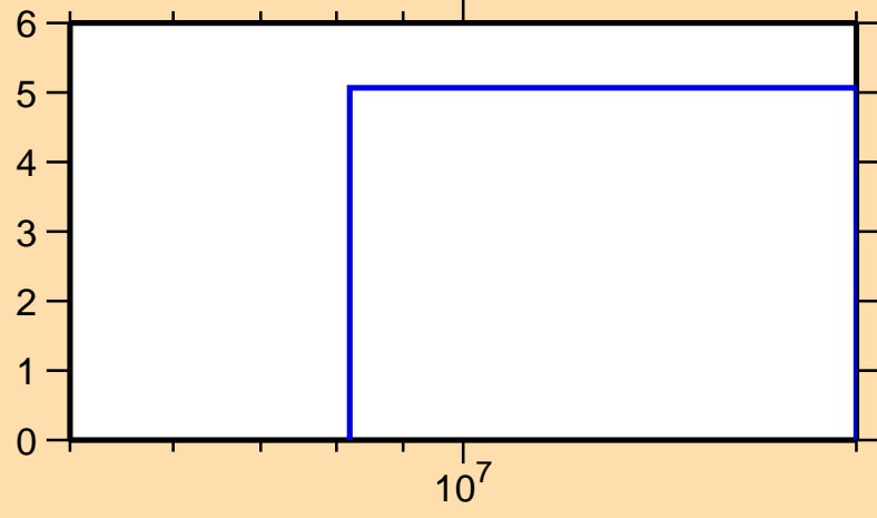
\Delta\sigma/\sigma vs. E for ^{153}\text{Tb}(n,\text{tot.})
