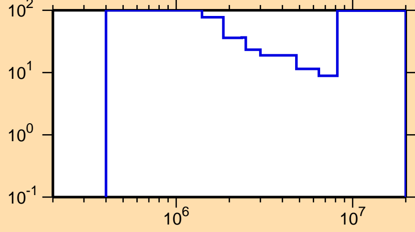
\Delta\sigma/\sigma vs. E for ^{153}\text{Tb}(n,n\text{cont.})
