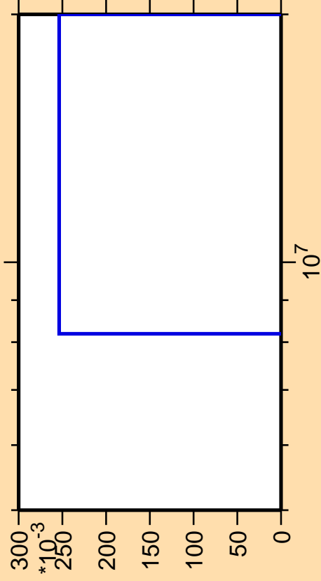
\Delta\sigma/\sigma vs. E for ^{153}\text{Tb}(n,3n\alpha)
