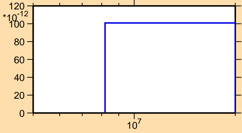
\sigma vs. E for ^{153}\text{Tb}(\text{mt } 45)
