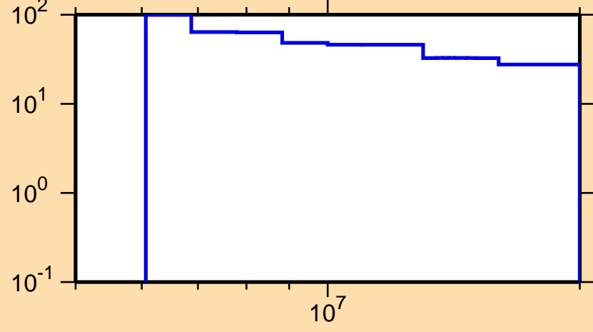
\Delta\sigma/\sigma vs. E for ^{154}\text{Tb}(n,2n)
