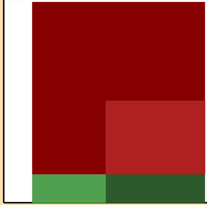
\Delta\sigma/\sigma vs. E for ^{154}\text{Tb}(n,2n)
