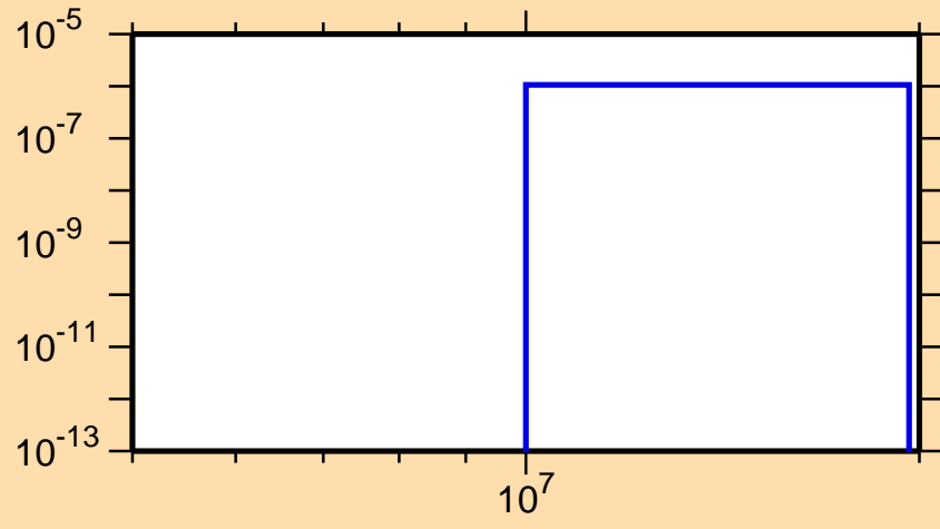
\sigma vs. E for ^{154}\text{Tb}(n,2n\alpha)
