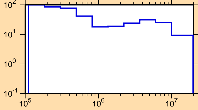
\Delta\sigma/\sigma vs. E for ^{154}\text{Tb}(n,\text{el.})
