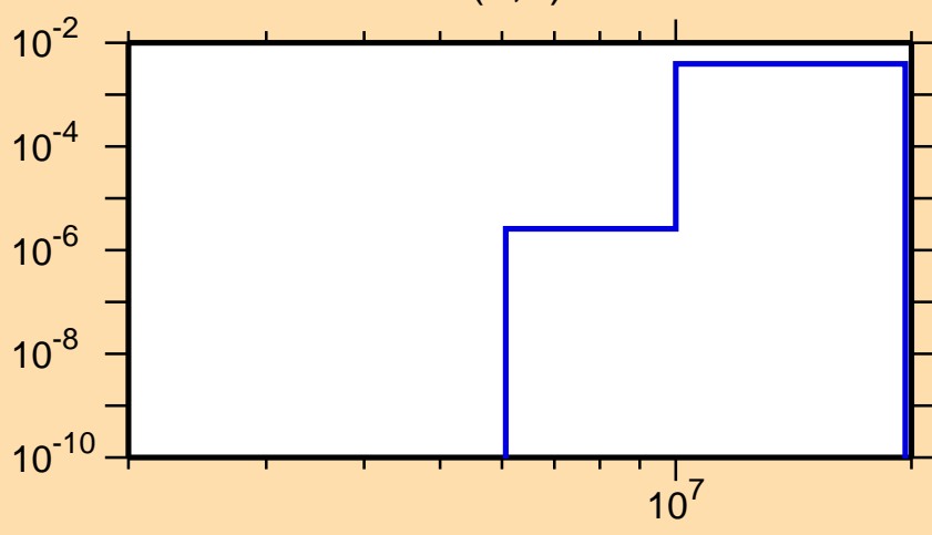
\sigma vs. E for ^{154}\text{Tb}(n,d)
