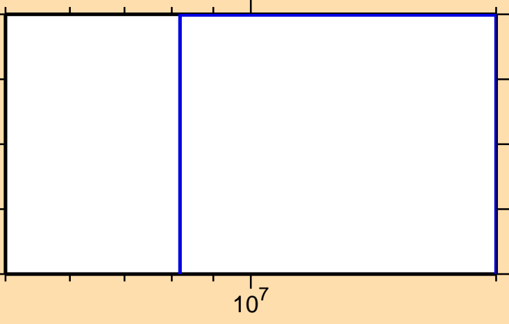
\sigma vs. E for ^{154}\text{Tb}(n,3n)
