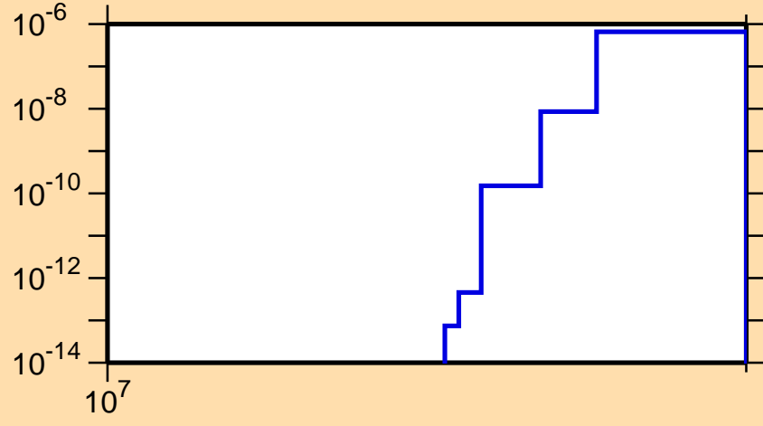
\sigma vs. E for ^{155}\text{Tb}(n,nt)
