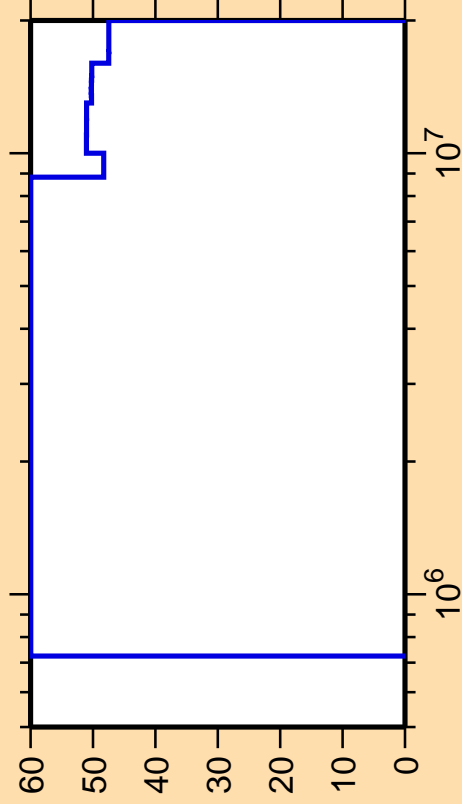
\Delta\sigma/\sigma vs. E for ^{155}\text{Tb}(n,p)
