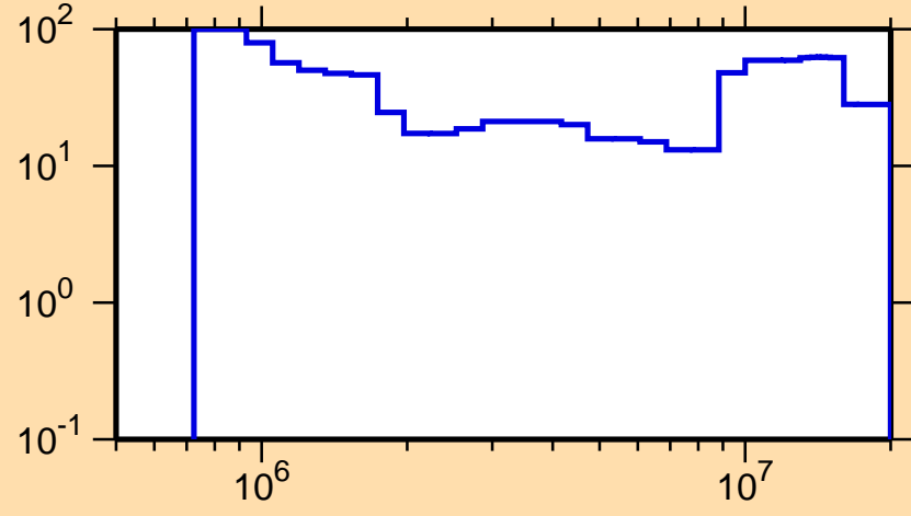
\Delta\sigma/\sigma vs. E for ^{155}\text{Tb}(n,ncont.)
