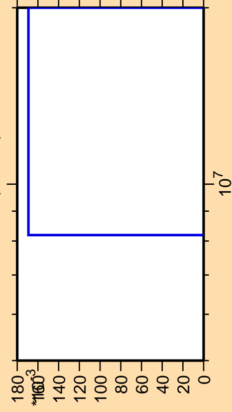
\Delta\sigma/\sigma vs. E for ^{155}\text{Tb} (mt 45)
