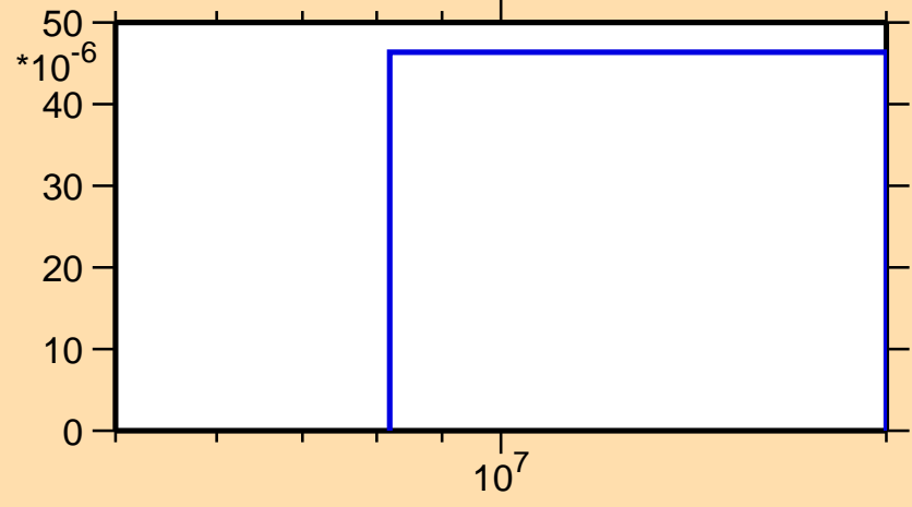
\sigma vs. E for ^{155}\text{Tb}(n,t)
