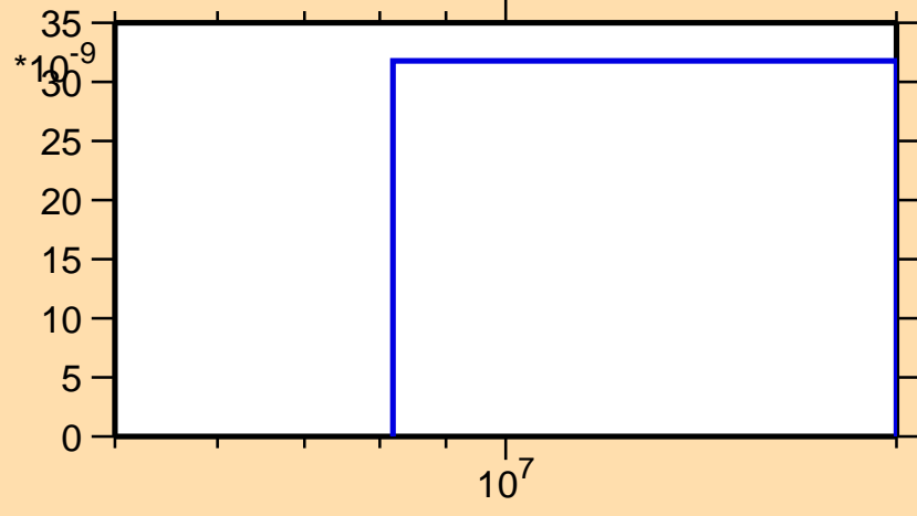
\sigma vs. E for ^{155}\text{Tb}(n,\text{nd})
