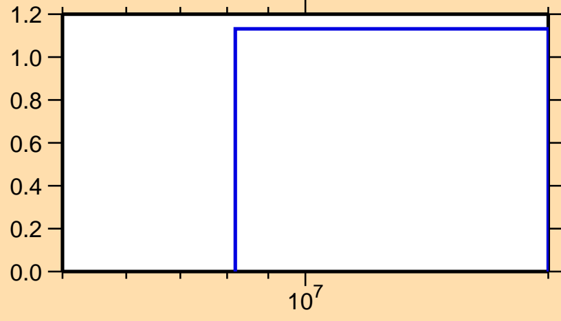
\sigma vs. E for ^{155}\text{Tb}(n,2n)
