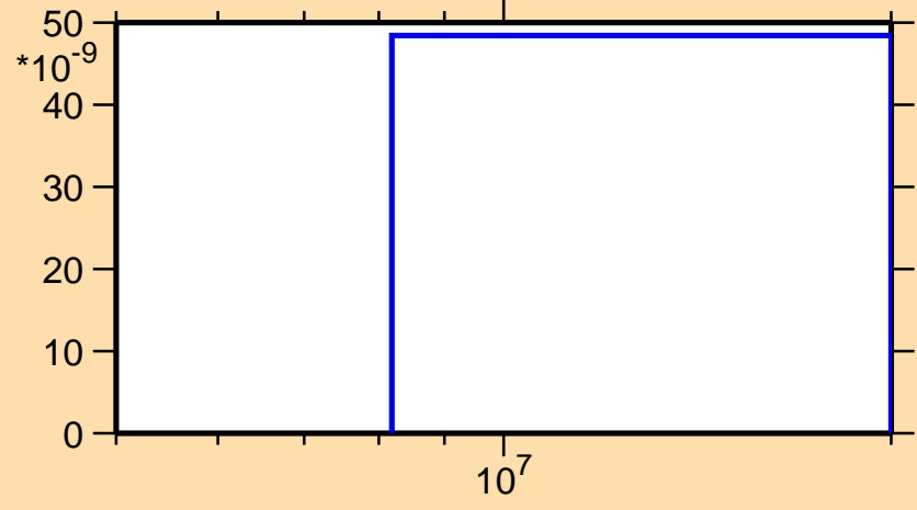
\sigma vs. E for ^{155}\text{Tb}(n,2np)
