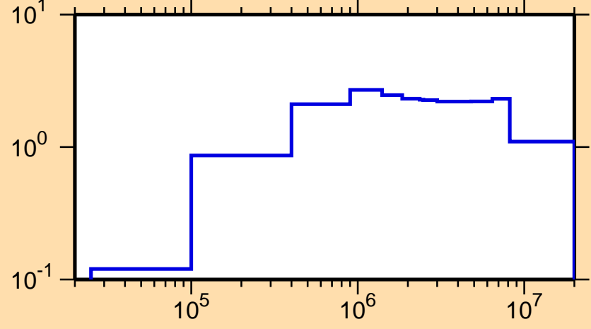
\sigma vs. E for ^{155}\text{Tb}(n,\text{inel.})
