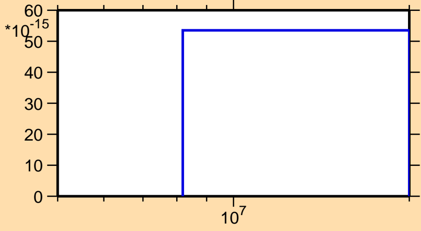
\sigma vs. E for ^{155}\text{Tb} (mt 45)
