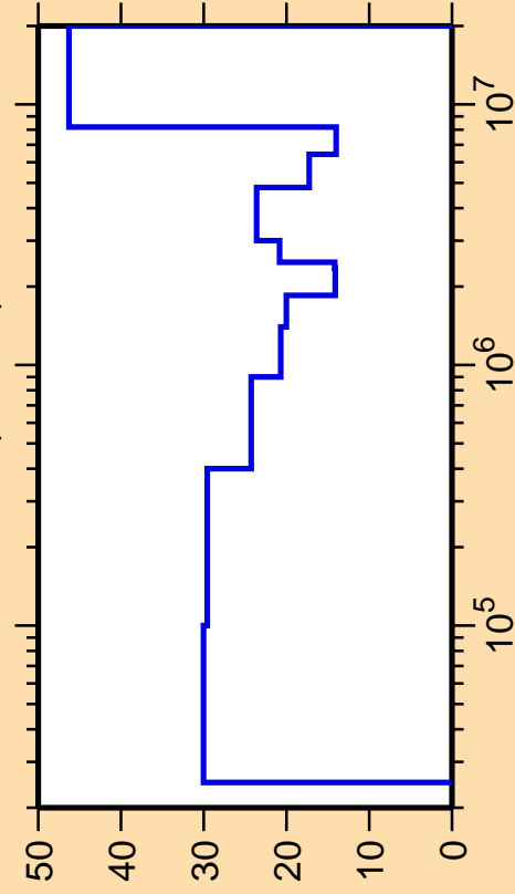
\Delta\sigma/\sigma vs. E for ^{155}\text{Tb}(n,\text{inel.})
