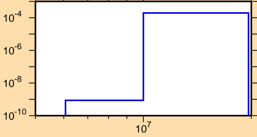
\sigma vs. E for ^{156}\text{Tb}(n,t)
