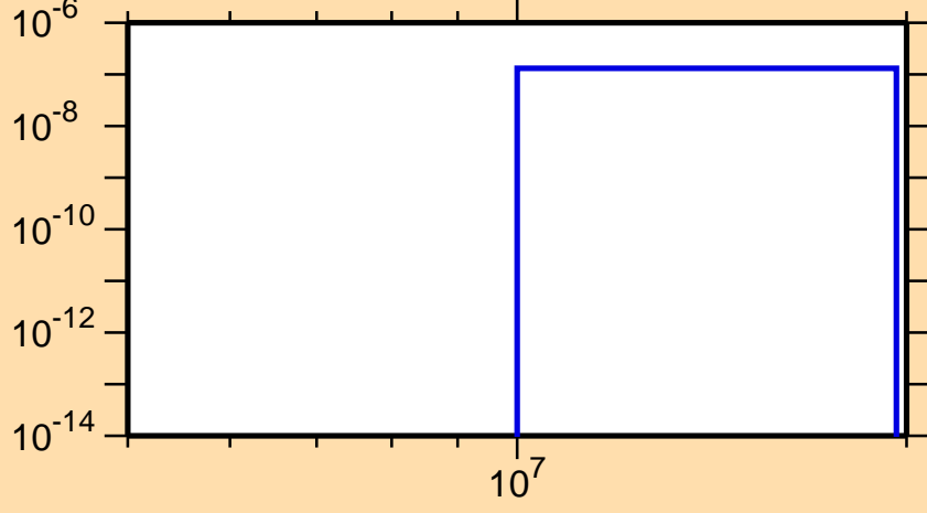
\sigma vs. E for ^{156}\text{Tb}(n,2n\alpha)
