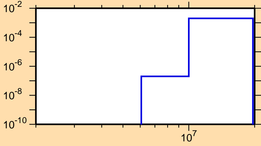
\sigma vs. E for ^{156}\text{Tb}(n,d)
