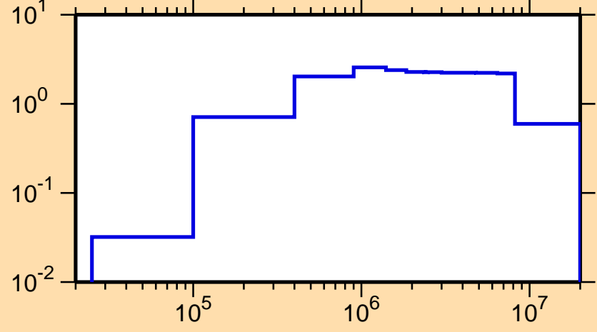
\sigma vs. E for ^{156}\text{Tb}(n,\text{inel.})
