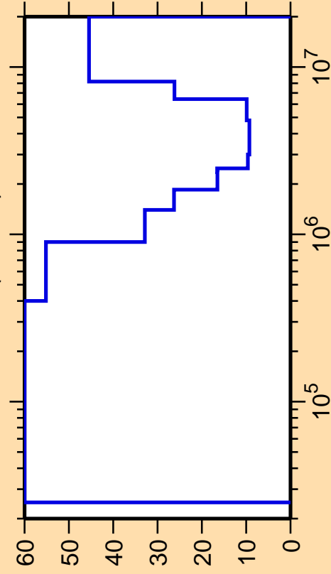
\Delta\sigma/\sigma vs. E for ^{156}\text{Tb}(n,\text{inel.})
