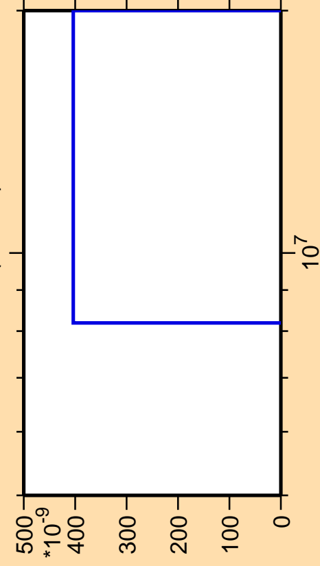
\Delta\sigma/\sigma vs. E for ^{156}\text{Tb}(\text{mt } 11)
