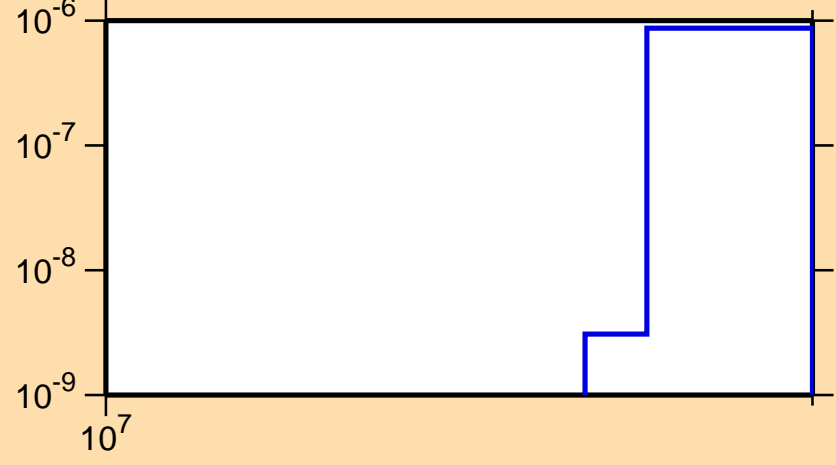
\sigma vs. E for ^{157}\text{Tb}(n,2np)
