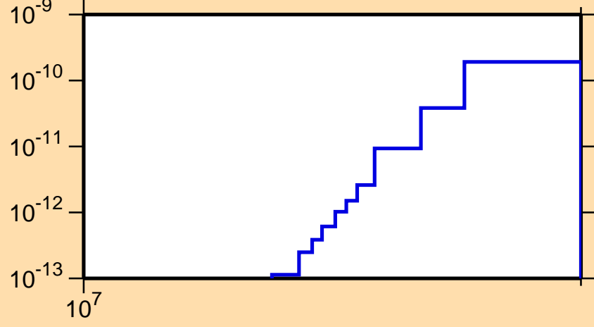
\sigma vs. E for ^{157}\text{Tb}(n,p\alpha)
