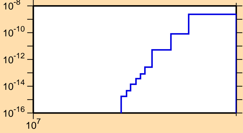
\sigma vs. E for ^{157}\text{Tb}(n,\text{He3})
