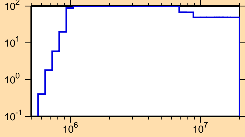
\Delta\sigma/\sigma vs. E for ^{157}\text{Tb}(n,p)
