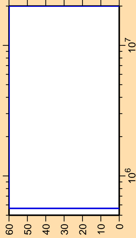
\Delta\sigma/\sigma vs. E for ^{157}\text{Tb}(n,\alpha)
