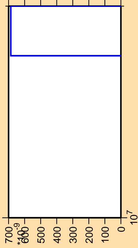
\Delta\sigma/\sigma vs. E for ^{157}\text{Tb} (mt 11)
