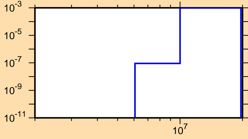
\sigma vs. E for ^{157}\text{Tb}(n,d)
