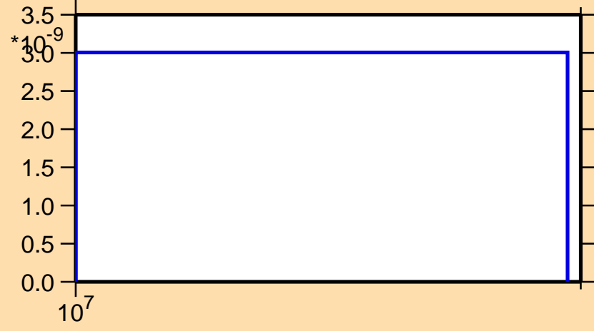
\sigma vs. E for ^{157}\text{Tb}(n,nt)
