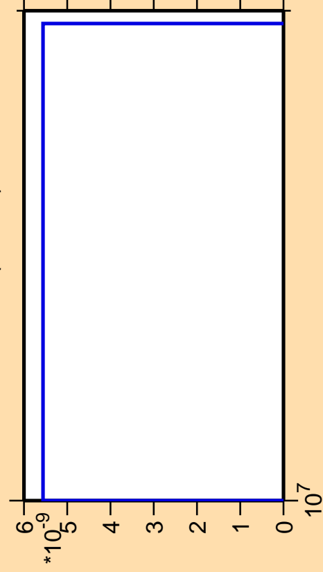
\Delta\sigma/\sigma vs. E for ^{157}\text{Tb} (mt 11)
