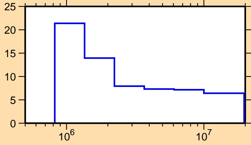
\Delta\sigma/\sigma vs. E for ^{157}\text{Tb}(n,n\text{nonel.})
