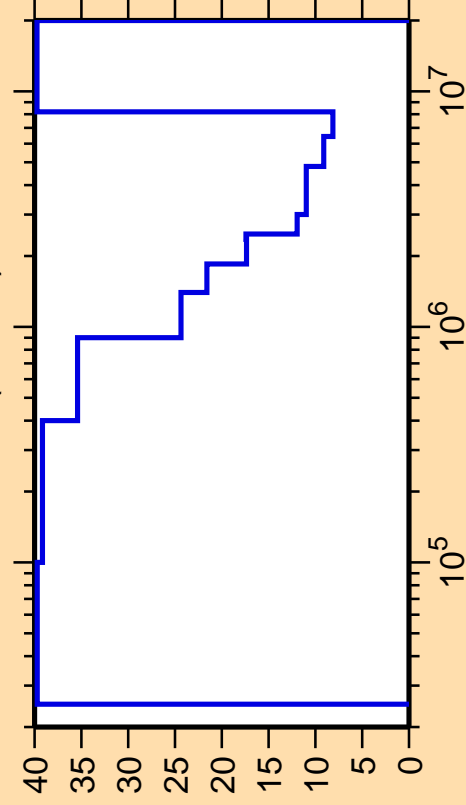
\Delta\sigma/\sigma vs. E for ^{157}\text{Tb}(n,\text{inel.})
