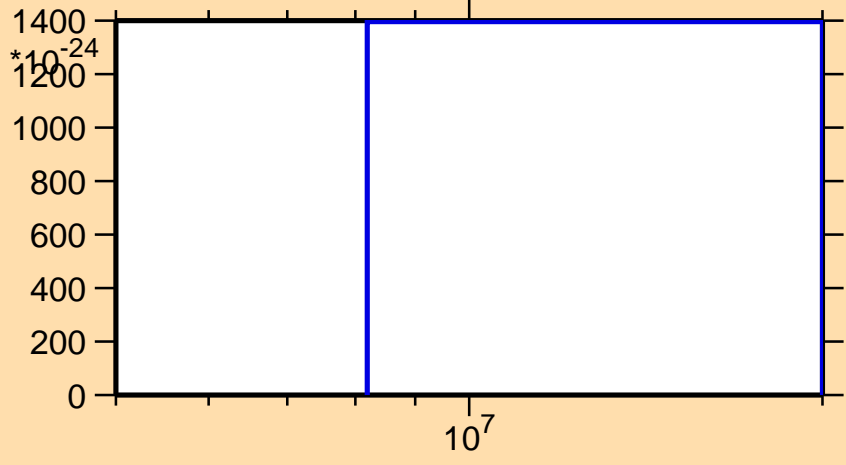
\sigma vs. E for ^{157}\text{Tb} (mt 11)
