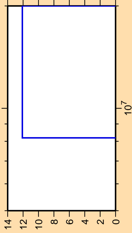
\Delta\sigma/\sigma vs. E for ^{157}\text{Tb}(n,2n)
