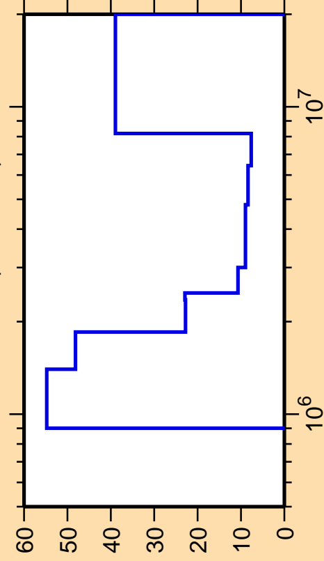
\Delta\sigma/\sigma vs. E for ^{157}\text{Tb}(n,\text{ncont.})
