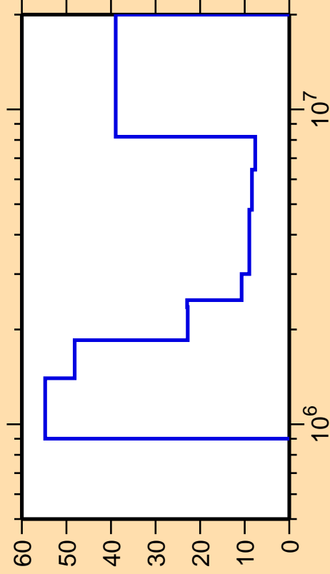
\Delta\sigma/\sigma vs. E for ^{157}\text{Tb}(n,n\text{cont.})
