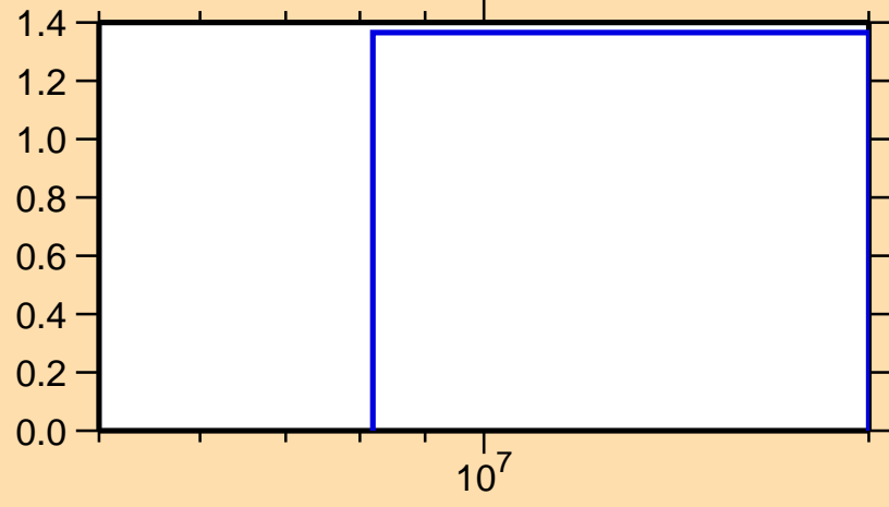
\sigma vs. E for ^{157}\text{Tb}(n,2n)
