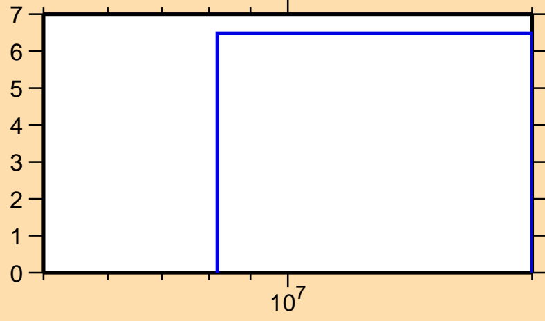
\Delta\sigma/\sigma vs. E for ^{157}\text{Tb}(n,\text{el.})
