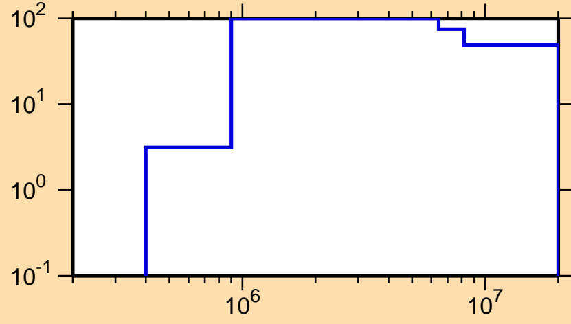
\Delta\sigma/\sigma vs. E for ^{157}\text{Tb}(n,p)
