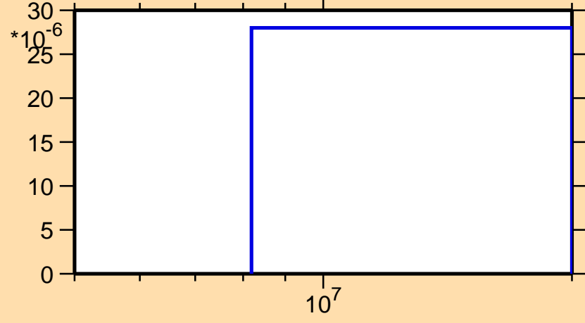
\sigma vs. E for ^{157}\text{Tb}(n,t)
