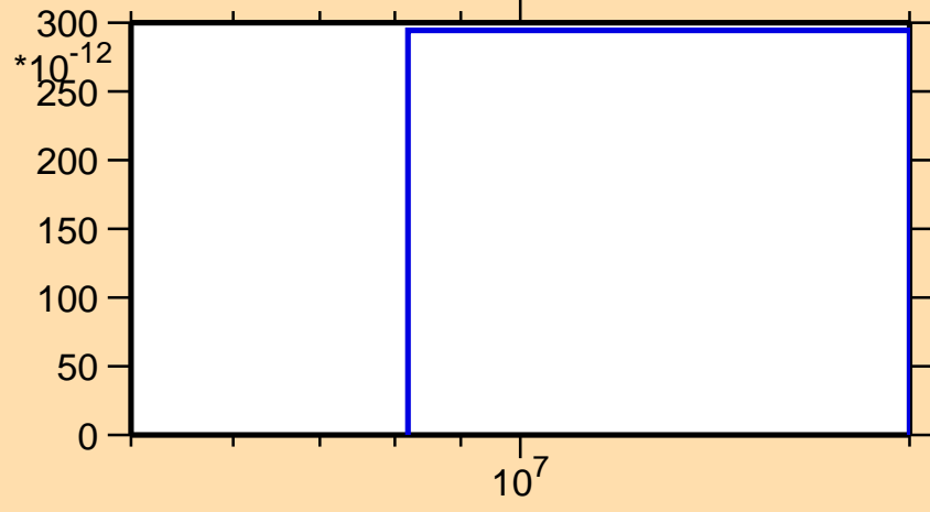
\sigma vs. E for ^{157}\text{Tb}(n,2n\alpha)
