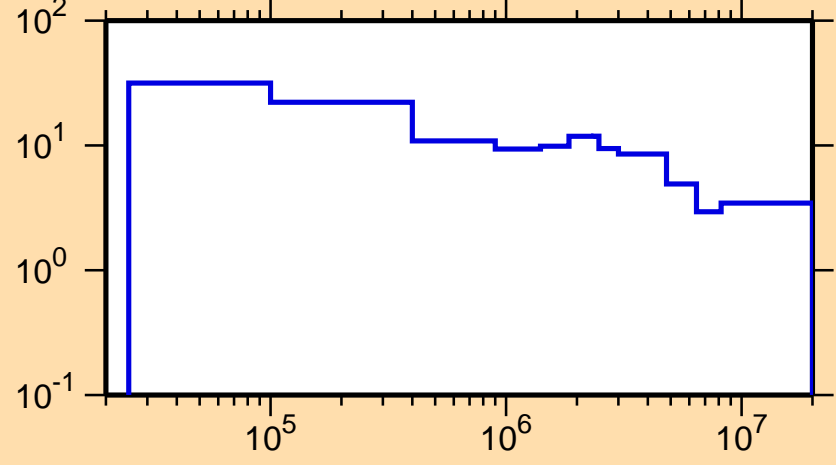
\Delta\sigma/\sigma vs. E for ^{157}\text{Tb}(n,\text{tot.})
