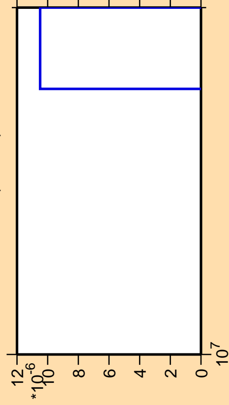
\Delta\sigma/\sigma vs. E for ^{158}\text{Tb} (mt 11)
