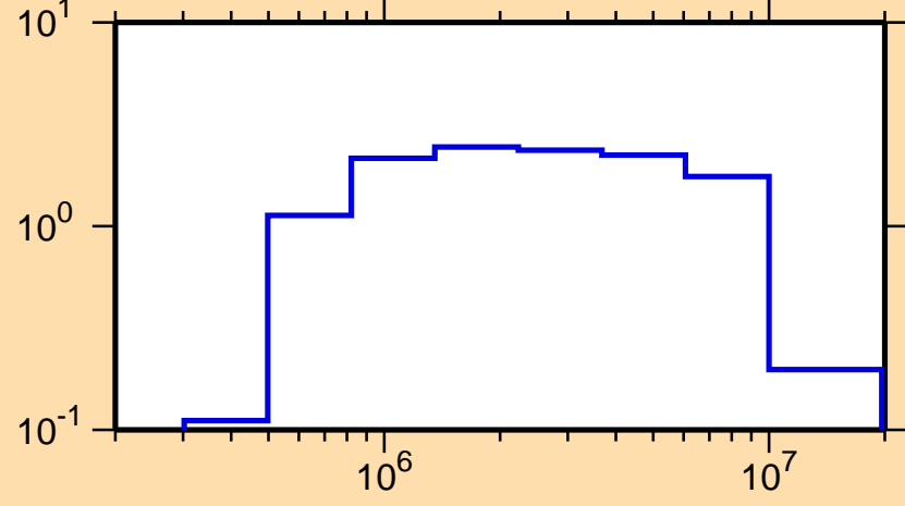
\sigma vs. E for ^{158}\text{Tb}(n,n\text{cont.})
