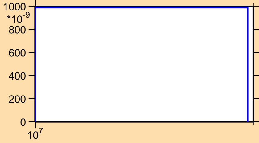
\sigma vs. E for ^{158}\text{Tb}(n,nd)
