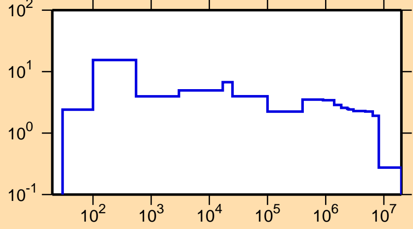
\sigma vs. E for ^{158}\text{Tb}(n,\text{inel.})
