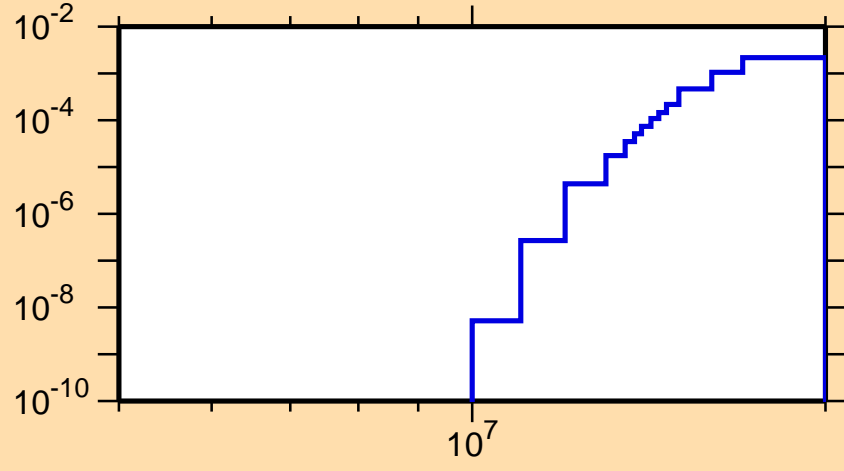
\sigma vs. E for ^{159}\text{Tb}(n,t)
