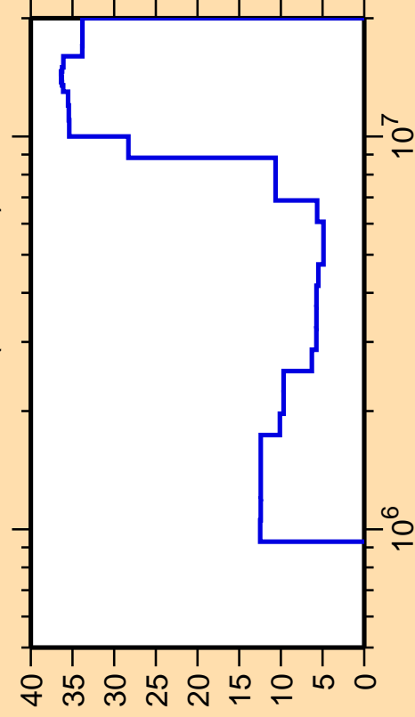
\Delta\sigma/\sigma vs. E for ^{159}\text{Tb}(n,\text{ncont.})
