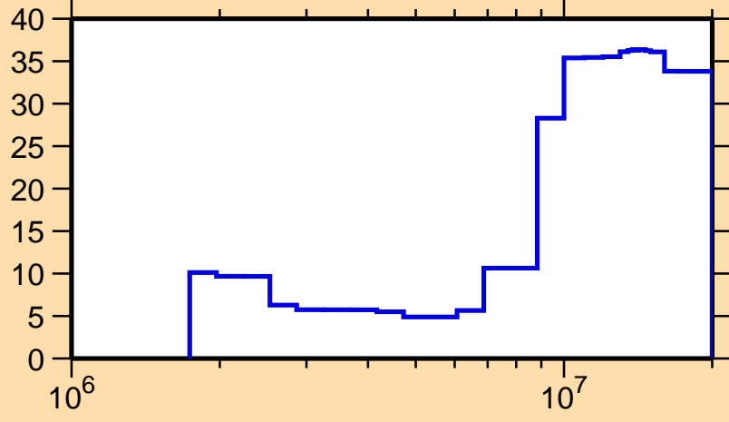
\Delta\sigma/\sigma vs. E for ^{159}\text{Tb}(n,n\text{cont.})
