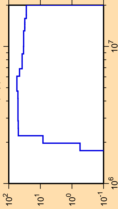
\Delta\sigma/\sigma vs. E for ^{159}\text{Tb}(n,p)
