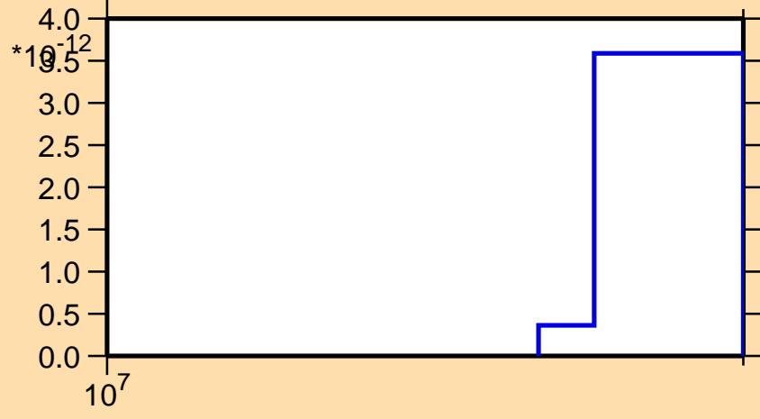
\sigma vs. E for ^{159}\text{Tb}(n,p\alpha)
