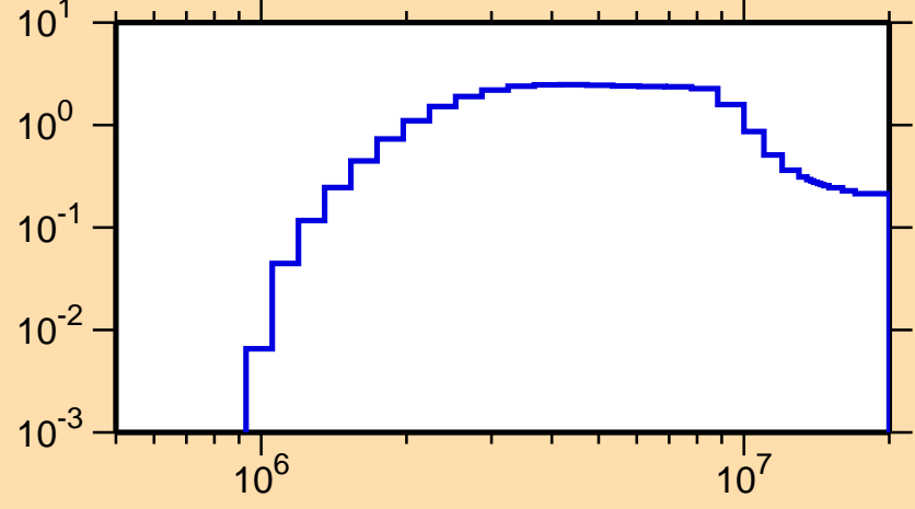
\sigma vs. E for ^{159}\text{Tb}(n,n\text{cont.})
