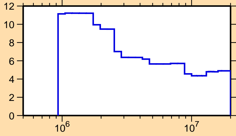
\Delta\sigma/\sigma vs. E for ^{159}\text{Tb}(n,n\text{onel.})
