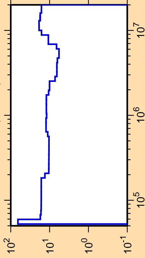
\Delta\sigma/\sigma vs. E for ^{159}\text{Tb}(n,\text{inel.})
