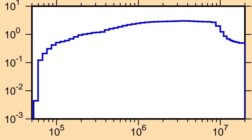
\sigma vs. E for ^{159}\text{Tb}(n,\text{inel.})
