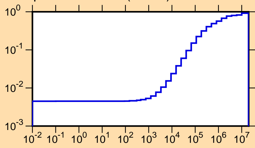
\mu vs. E for ^{159}\text{Tb}(\text{mt251})
