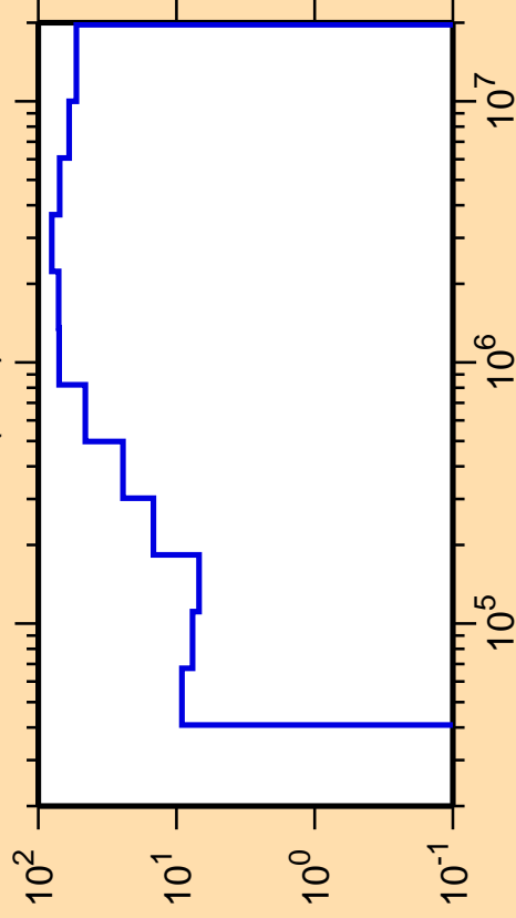
\Delta\sigma/\sigma vs. E for ^{159}\text{Tb}(n,\alpha)
