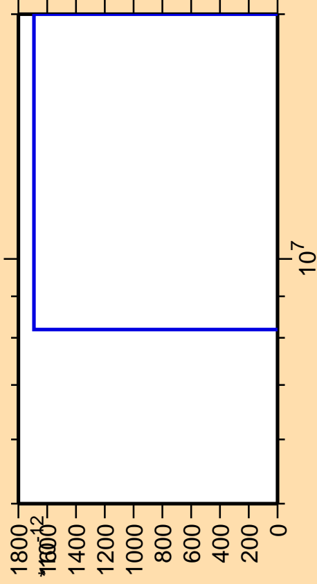
\Delta\sigma/\sigma vs. E for ^{159}\text{Tb}(\text{mt } 11)
