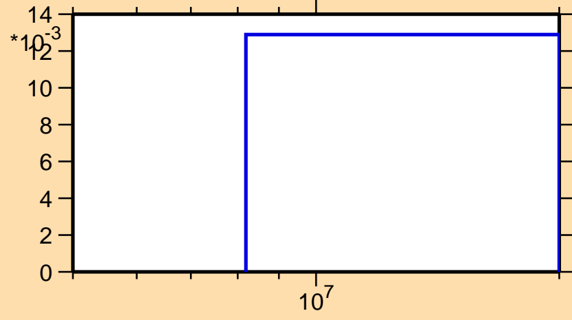
\sigma vs. E for ^{159}\text{Tb}(n,3n)
