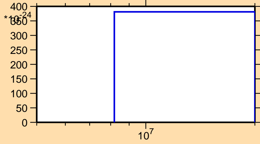
\sigma vs. E for ^{159}\text{Tb}(\text{mt } 11)
