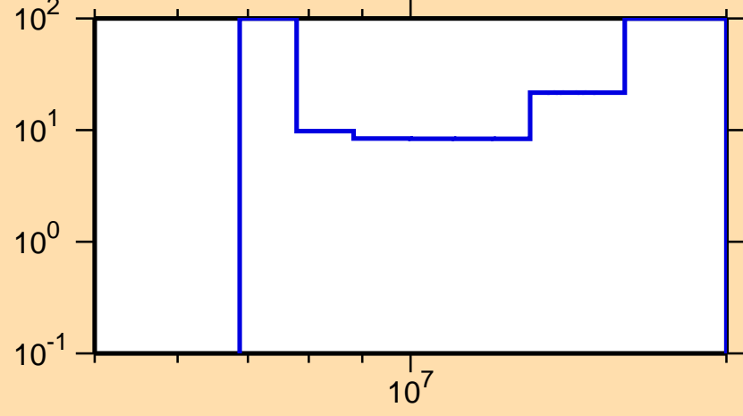
\Delta\sigma/\sigma vs. E for ^{161}\text{Tb}(n,2n)
