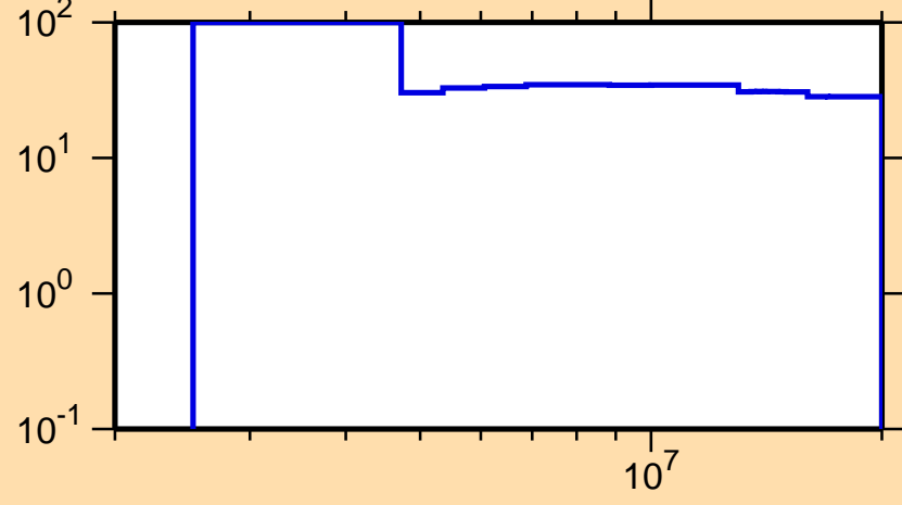
\Delta\sigma/\sigma vs. E for ^{161}\text{Tb}(n,n_1)
