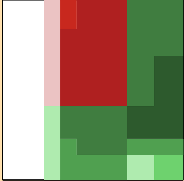
\Delta\sigma/\sigma vs. E for ^{161}\text{Tb}(n,2n)
