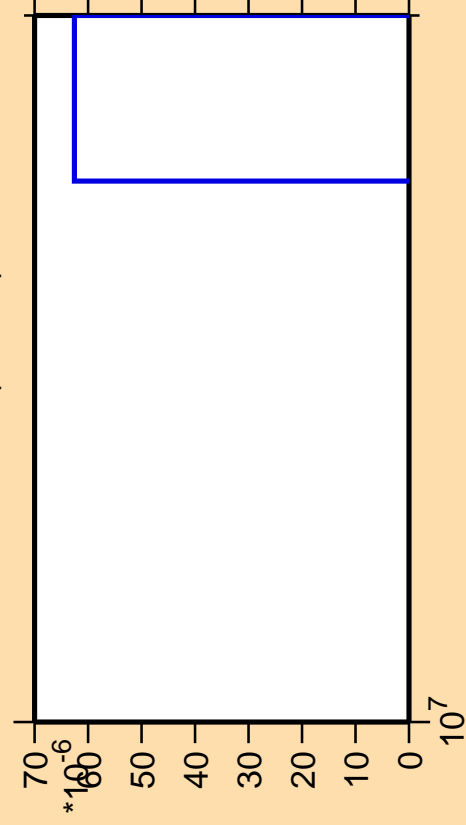
\Delta\sigma/\sigma vs. E for ^{161}\text{Tb} (mt 11)
